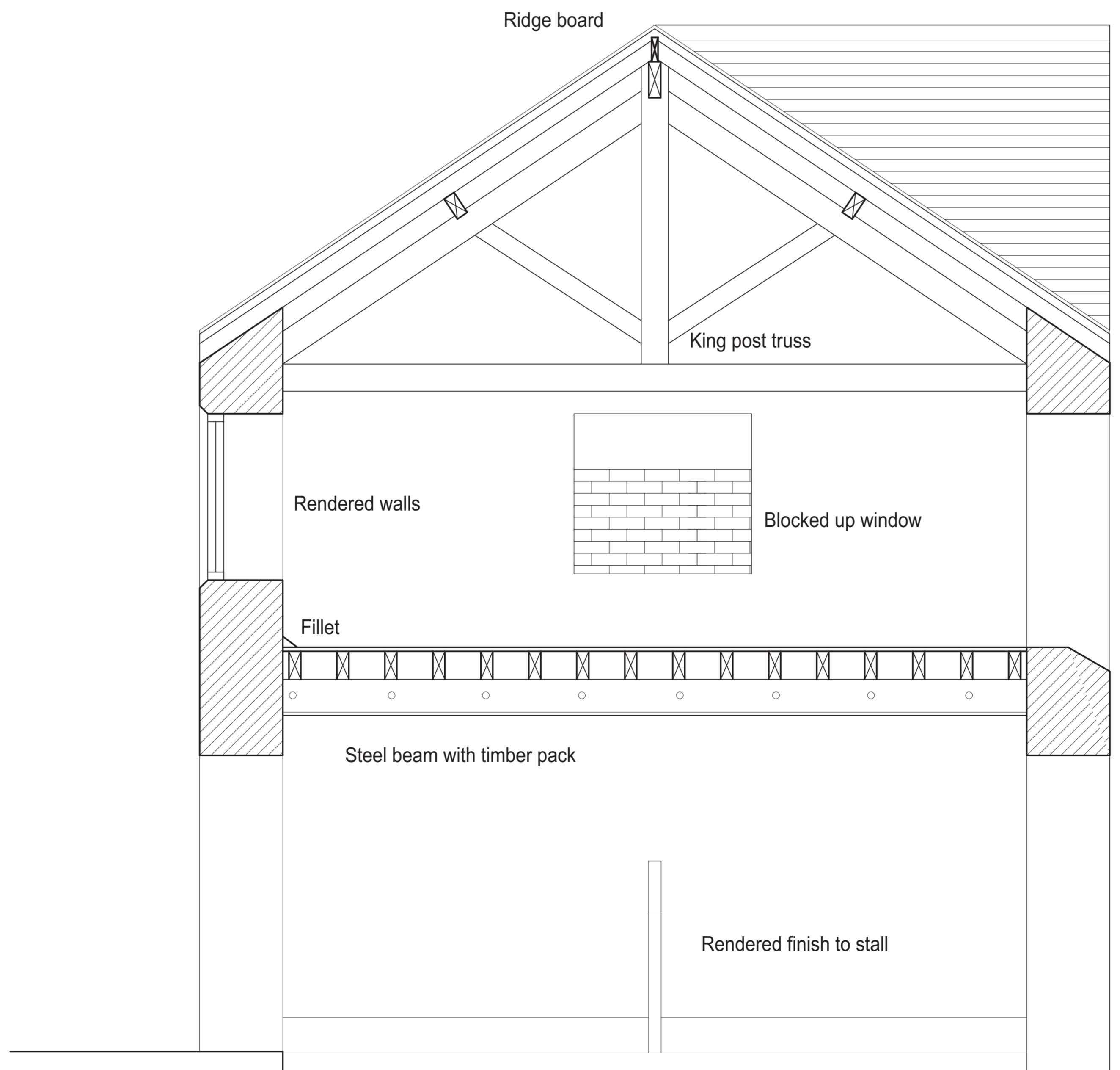
Section b-b
