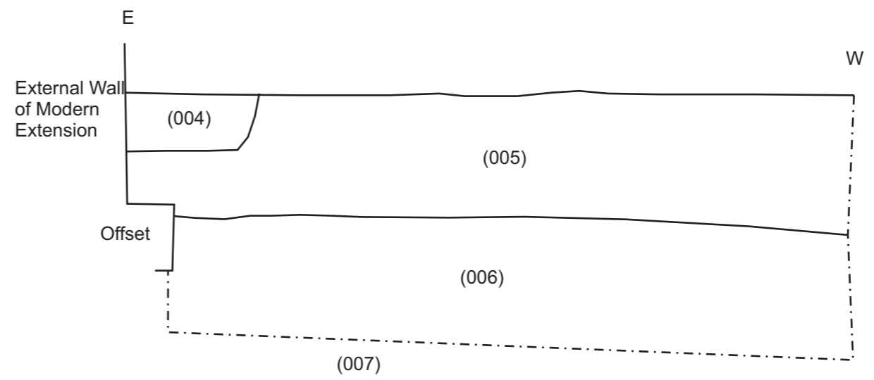
Representative Section 4, North Facing Section, Scale 1:20
