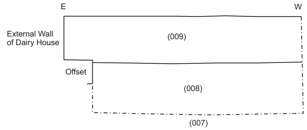
Representative Section 5, North Facing Section, Scale 1:20
