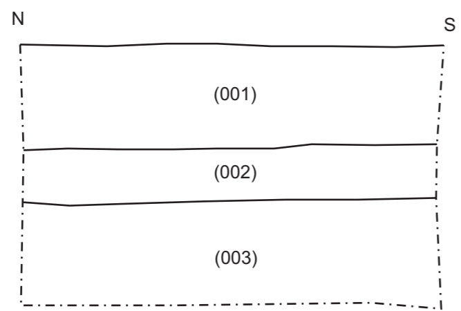
Representative Section 3, West Facing Section, Scale 1:20
