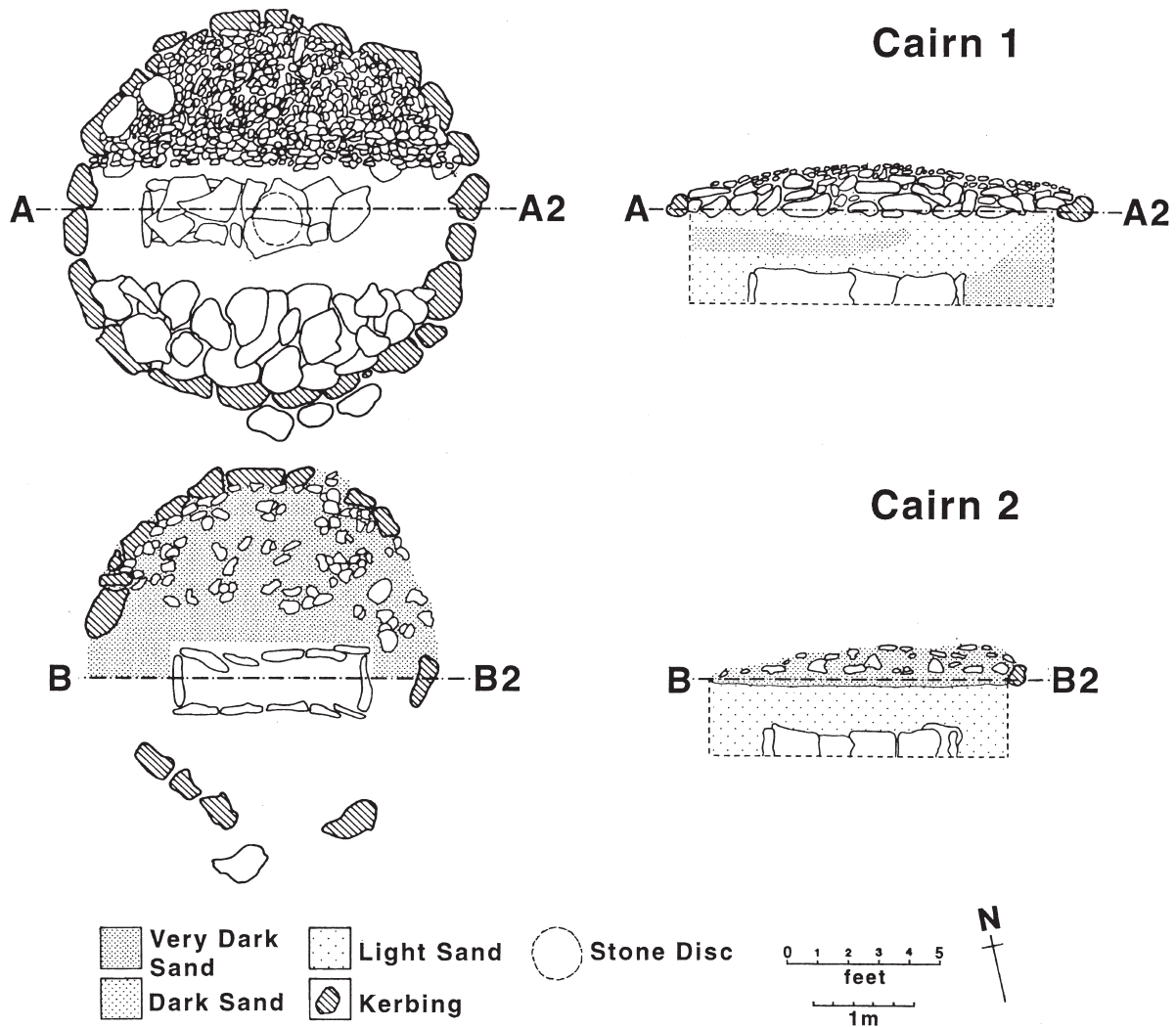
ILLUS 5 Plans of elevations of Cairns 1 and 2
