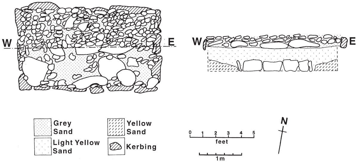
ILLUS 9 Plan and elevation of Rectangular Cairn 3
