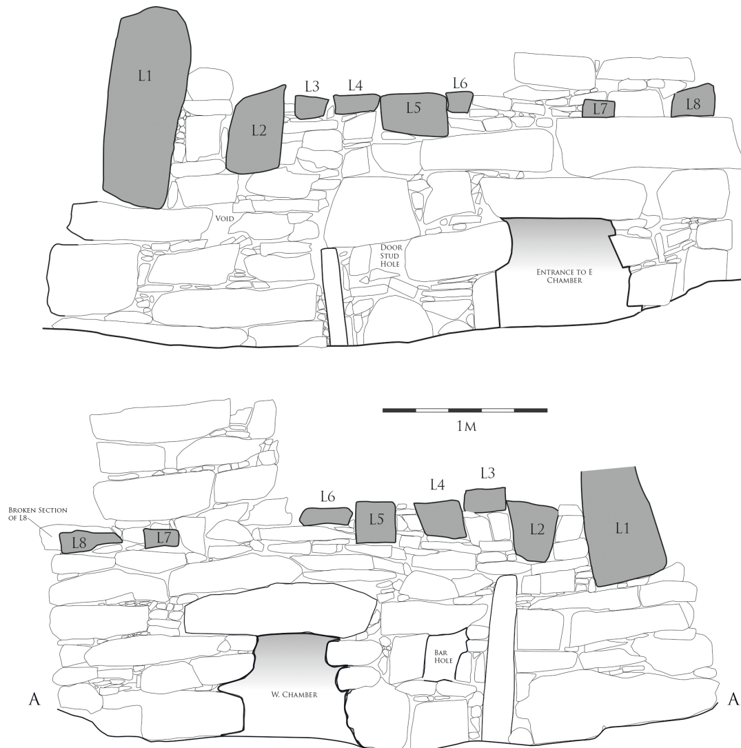
ILLUS 10 Elevations of the entrance to Clachtoll broch
