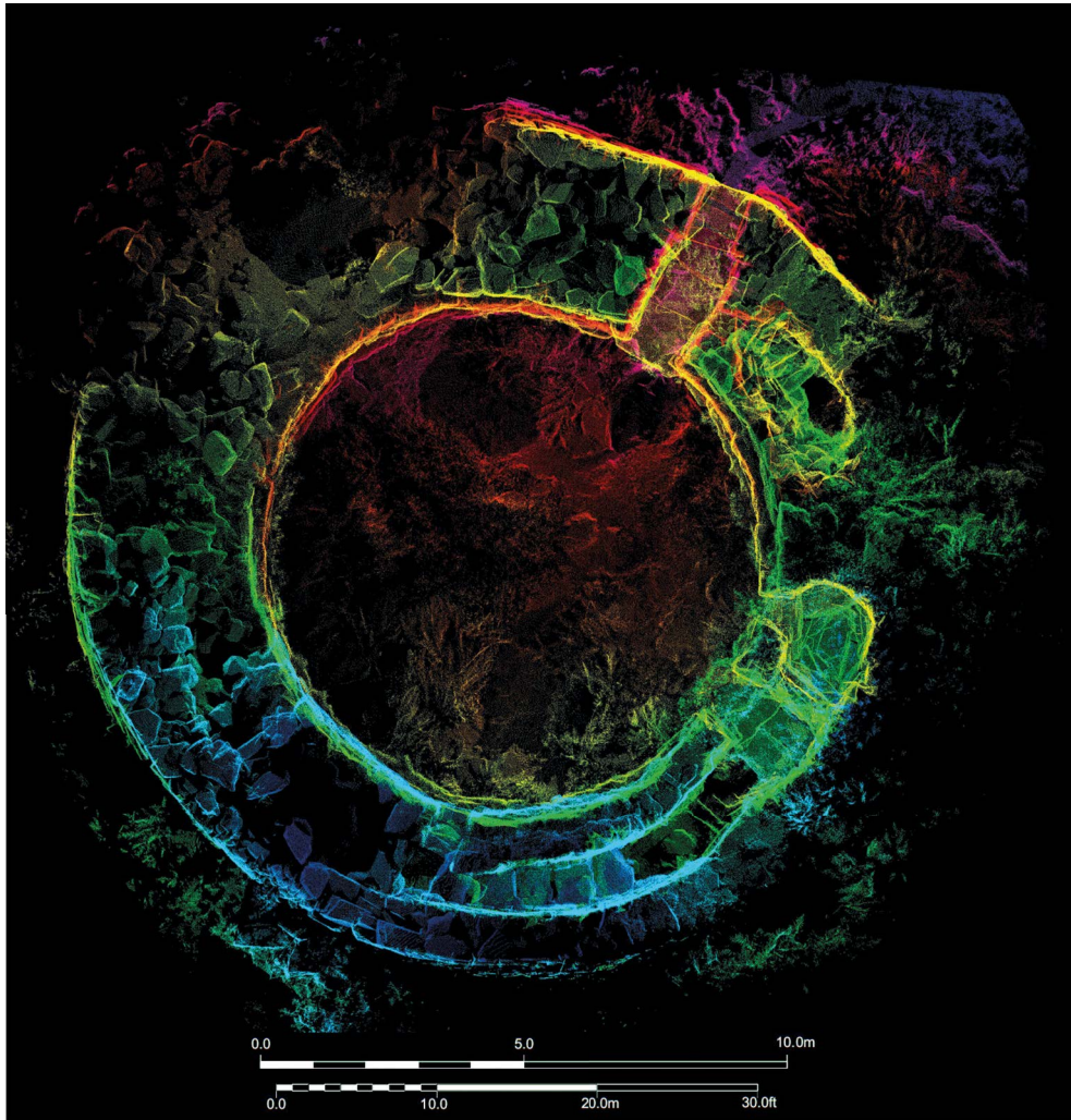
ILLUS 6 The orthographic plan of Caisteal Grugaig, derived from a laser scan, allows the depiction of the variable levels throughout the structure, and the position and heights of the intramural cells (purple/reds indicate low areas, light blue indicates high areas)
