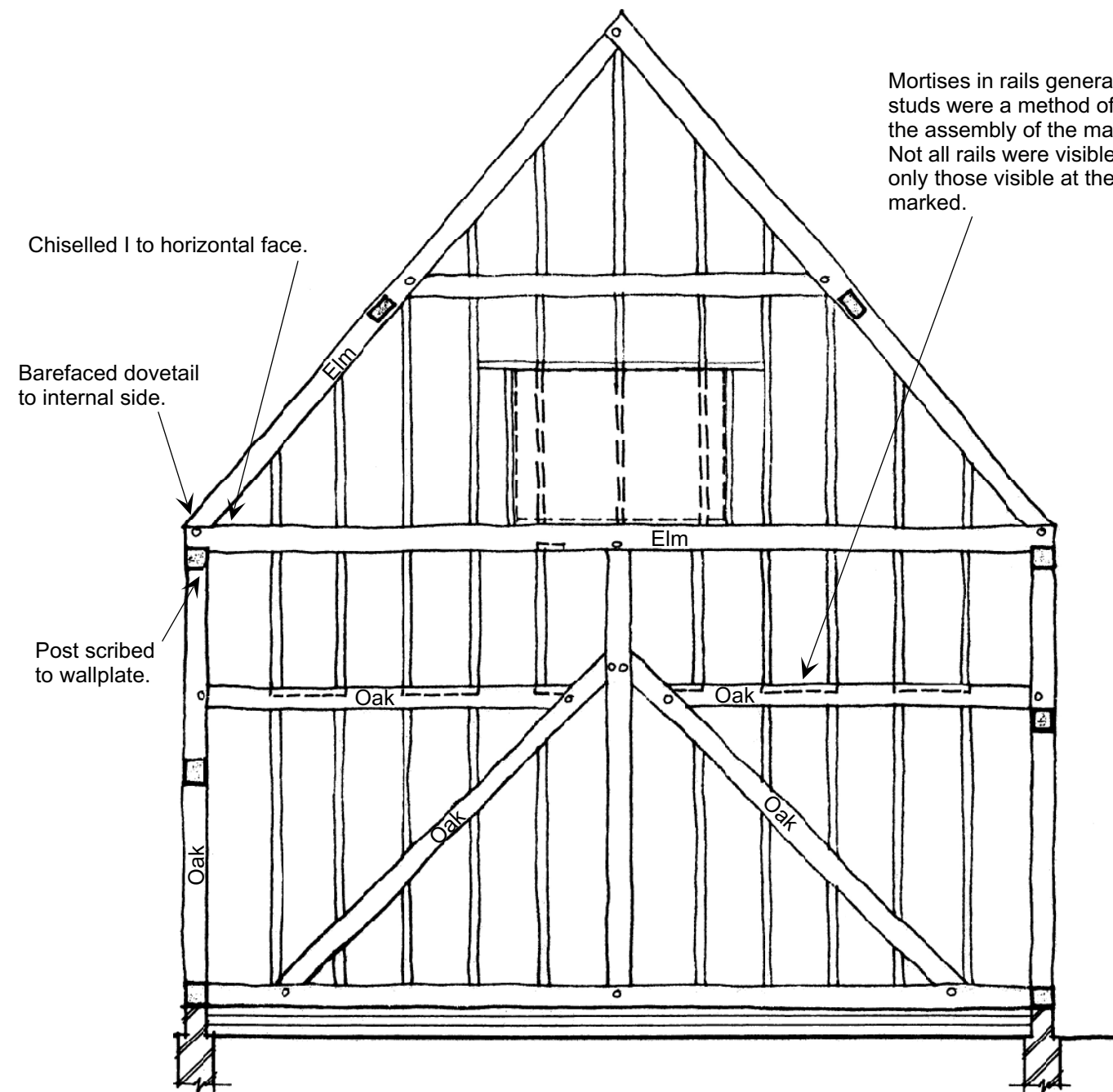
INTERNAL ELEVATION TOWARDS EAST.
