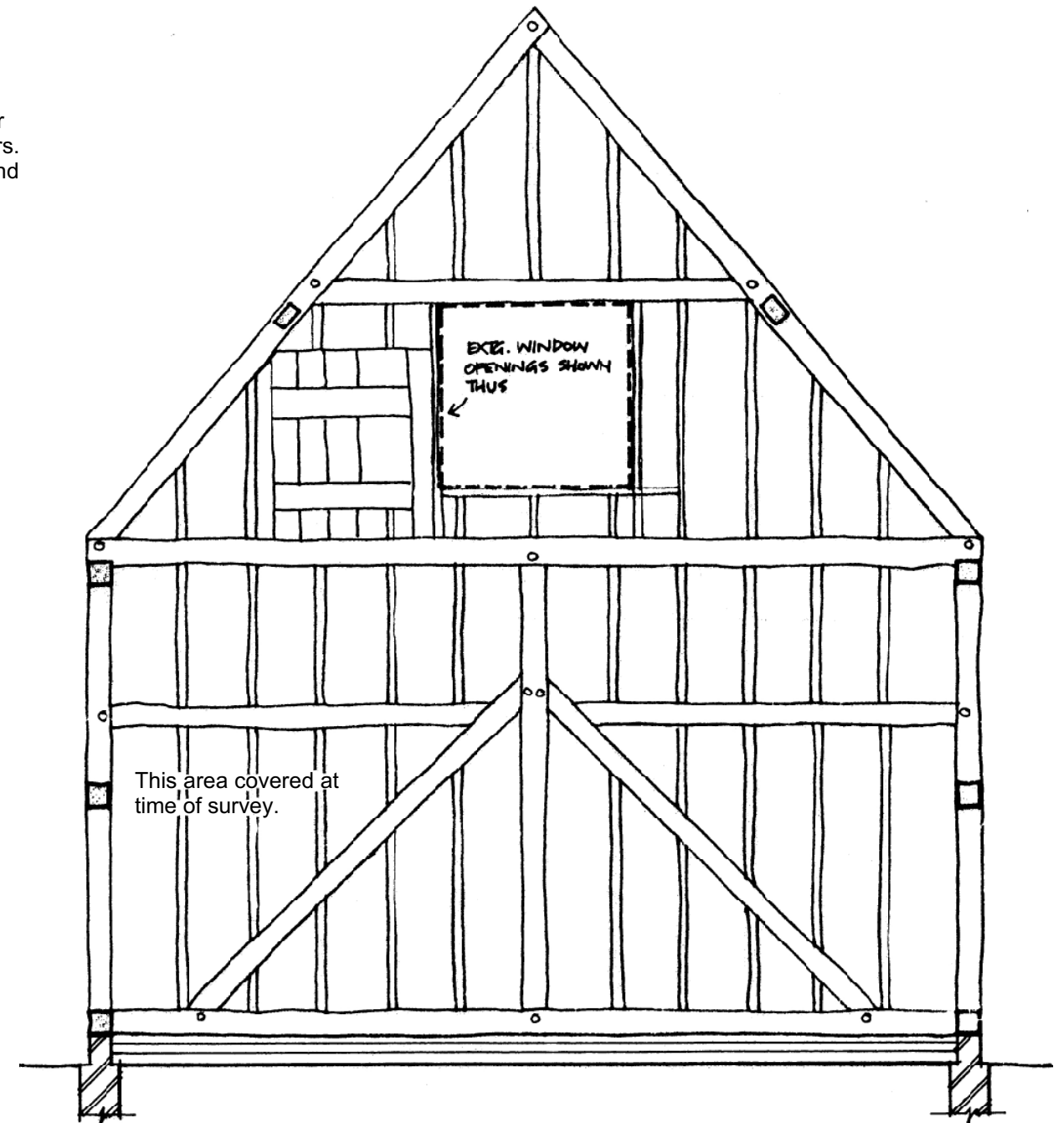
INTERNAL ELEVATION TOWARDS WEST
