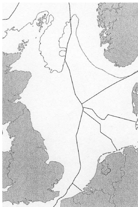
Fig 28 Map of the North sea basin showing areas of shallow water, which are the areas of highest potential for prehistoric human habitation (after Long et al 2004)
