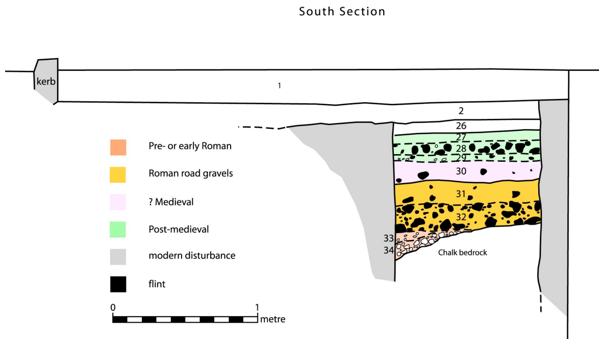
Figure 5: South section
