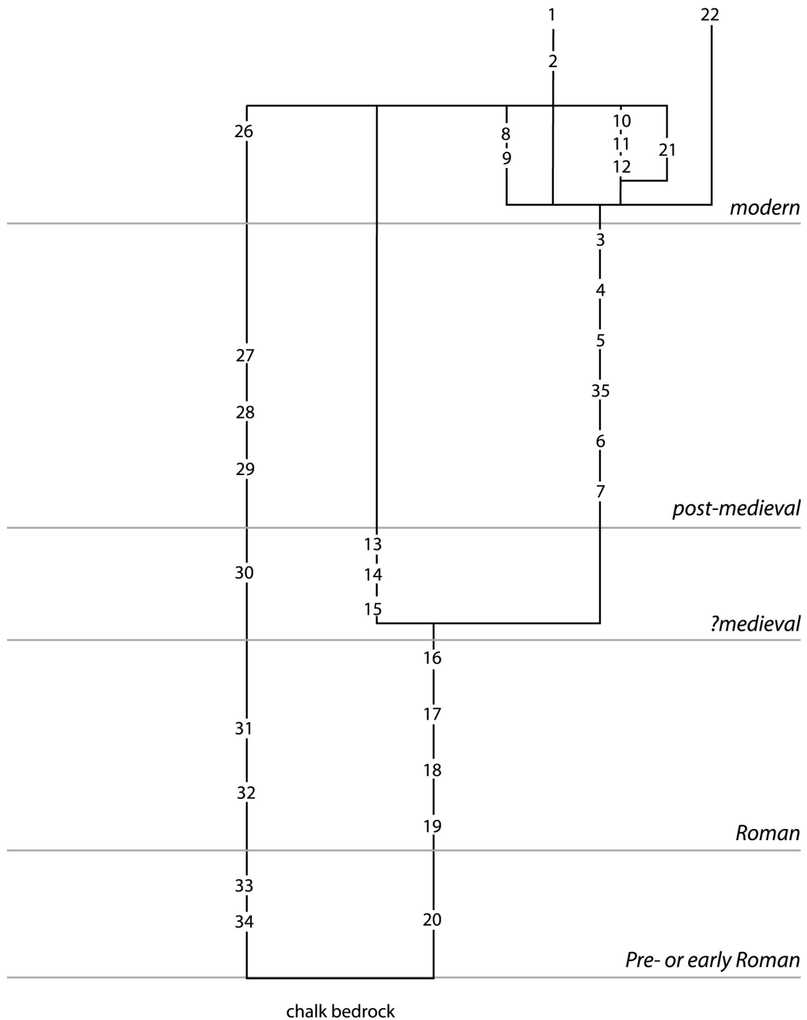
Figure 6: Stratigraphic Matrix
