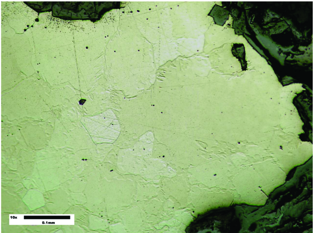
Plate 7.3.2 Effect of phosphorous on iron
