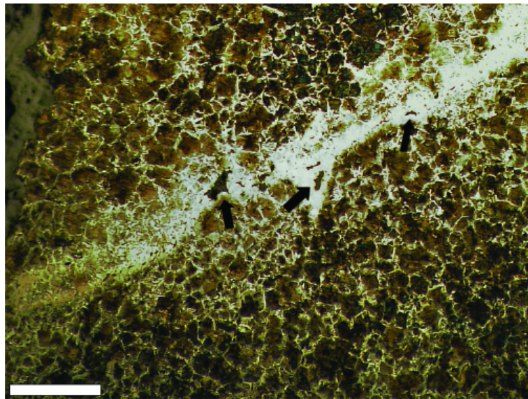
Plate 7.3.3 Weld lines
