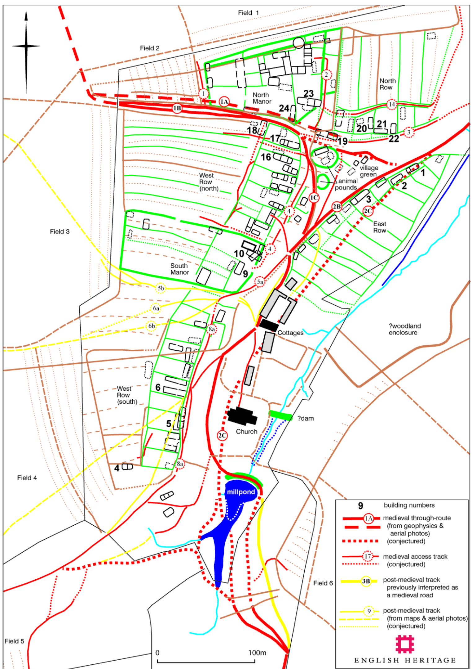
Fig 3.7 English Heritage schematic plan of the network of roads and tracks, at 1:1000 scale
