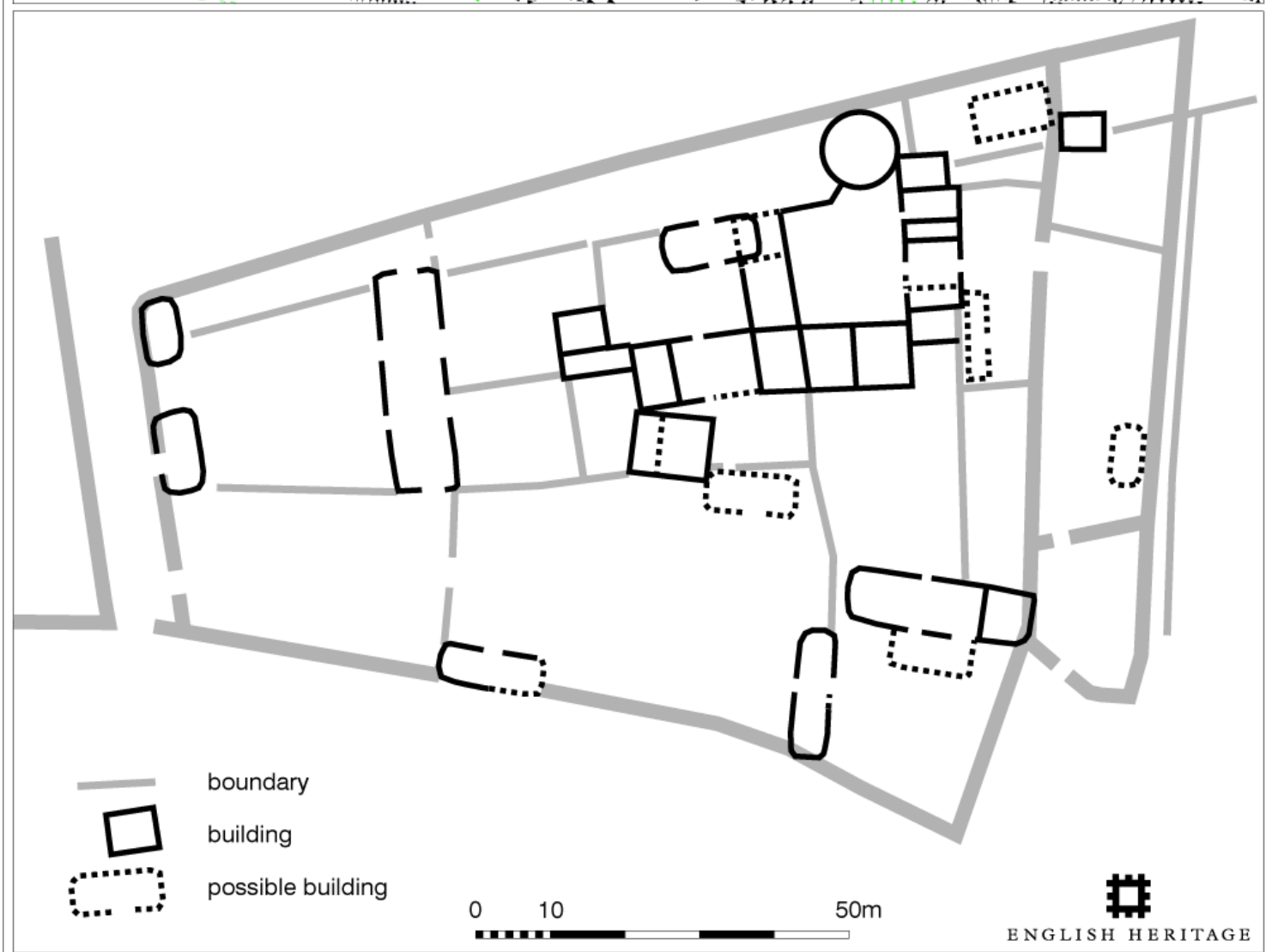
Fig 3.9 English Heritage plan of the North Manor (reduced from original at 1:500 scale), with schematic plan, without phasing
