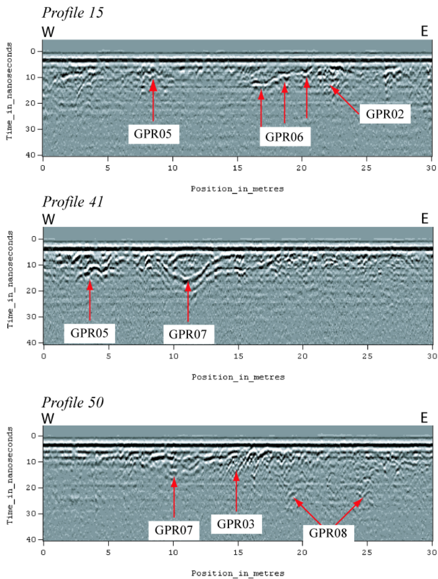
Fig 2.12 Representative profiles from the trial ground penetrating radar survey indicating significant anomalies identified in the amplitude time slices (see Figure 2.13).
