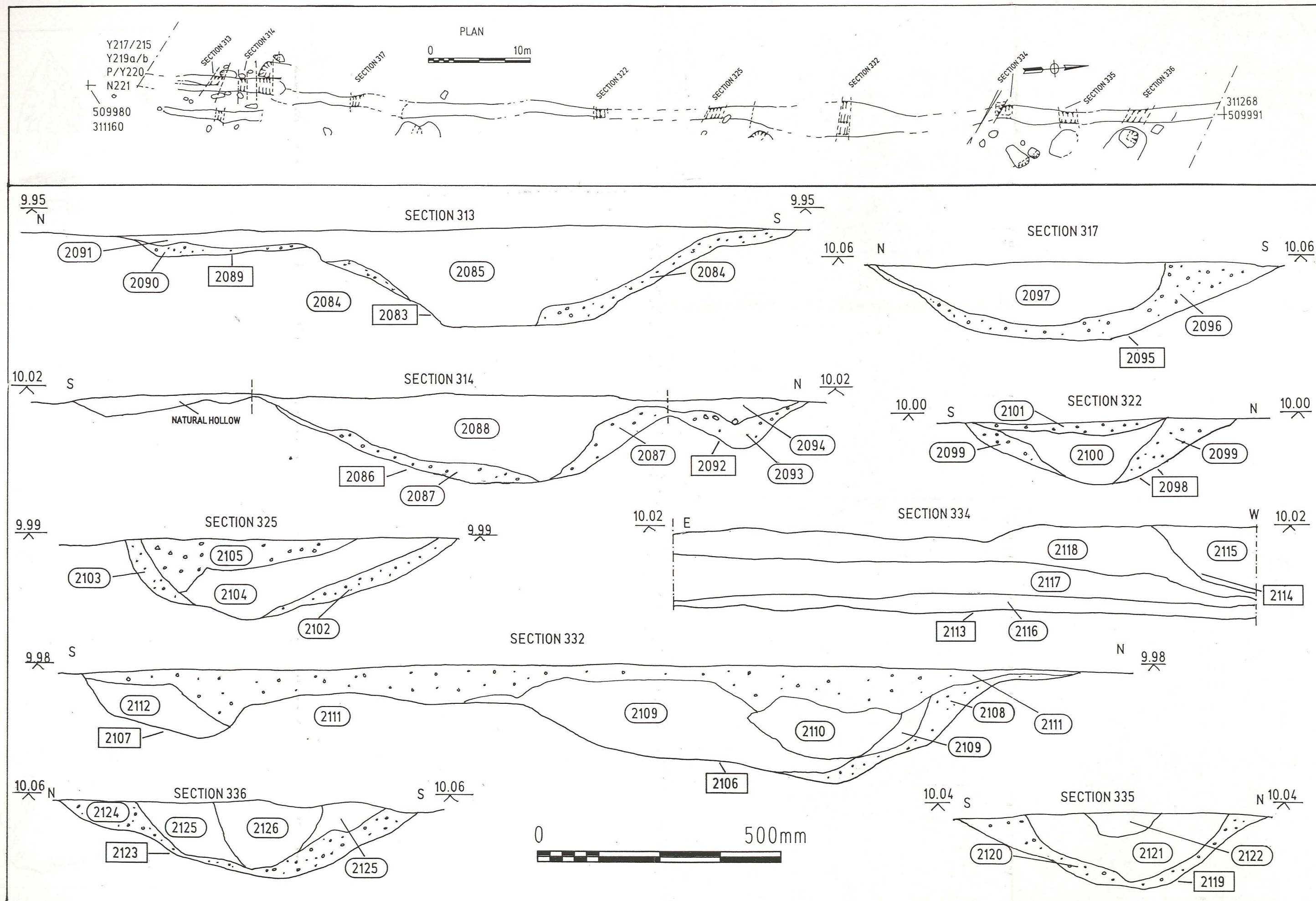
Figure 14: Ditch Y217 and Sections along its length
