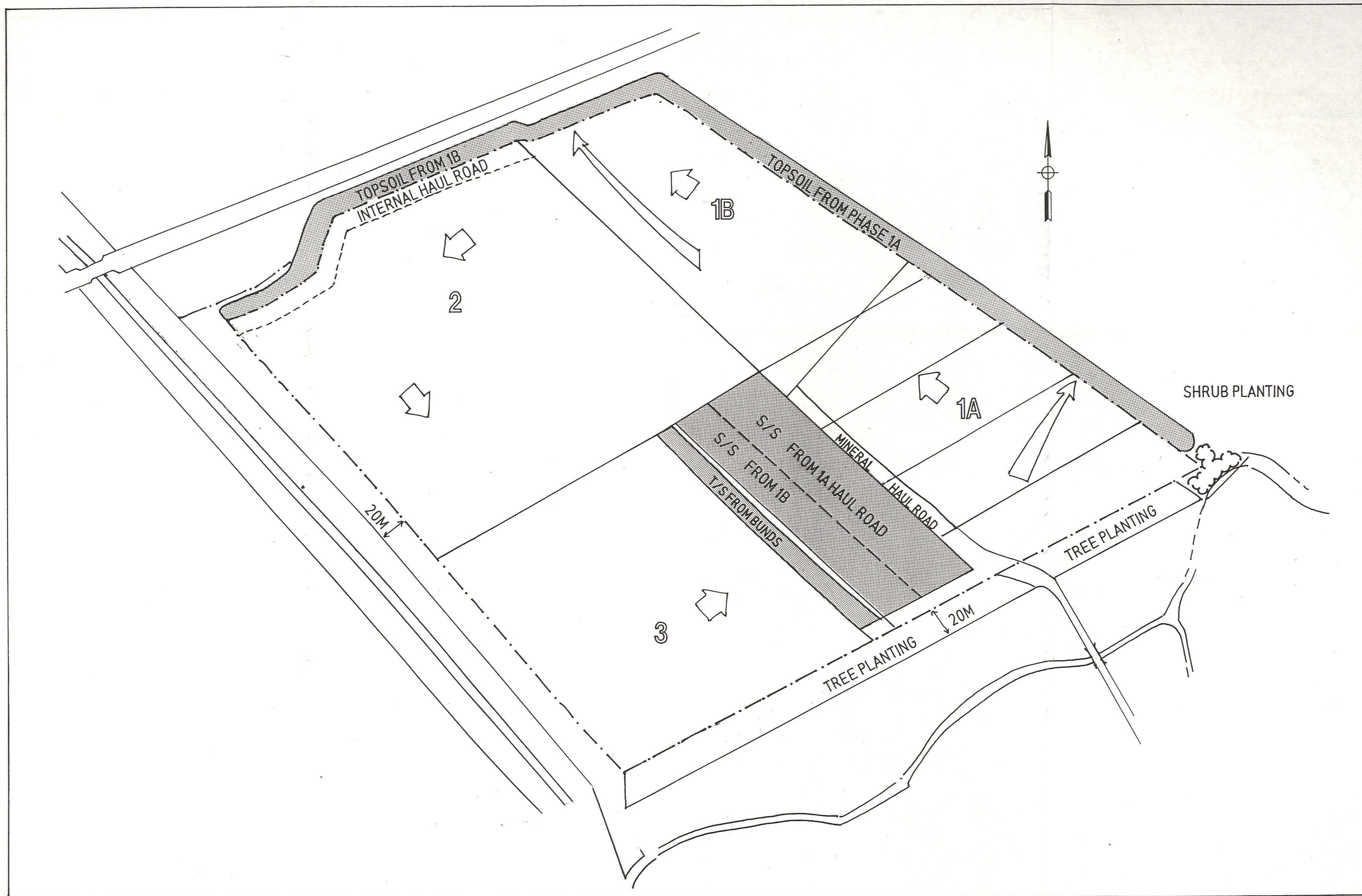
Figure 2: Amendment to extraction areas, bunds and subsoil dumping area
