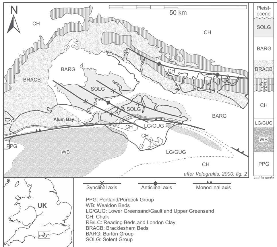
Figure 10. The geological context of Alum Bay (after Velagrakis, 2000: fig. 2).
