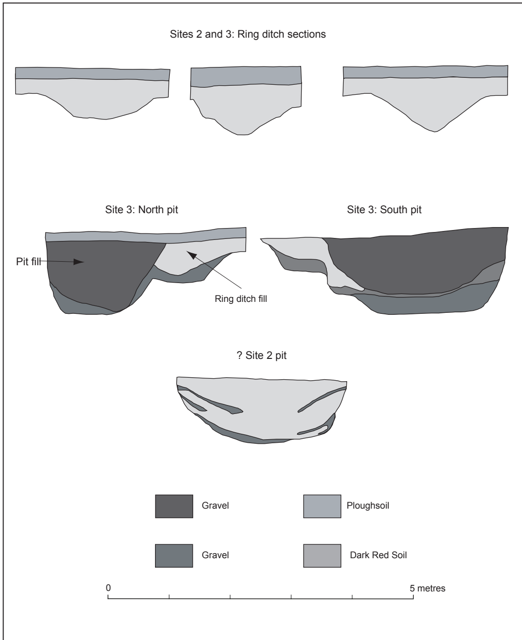
Figure 10: Sections from Netherhills Sites 2 and 3, redrawn from the Atkinson archive
