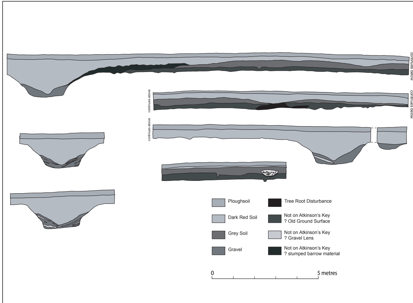
Figure 6: Section from Netherhills Site 1, redrawn from the Atkinson archive. Long section presumed to be north-east facing along Perryway, others unlocated
