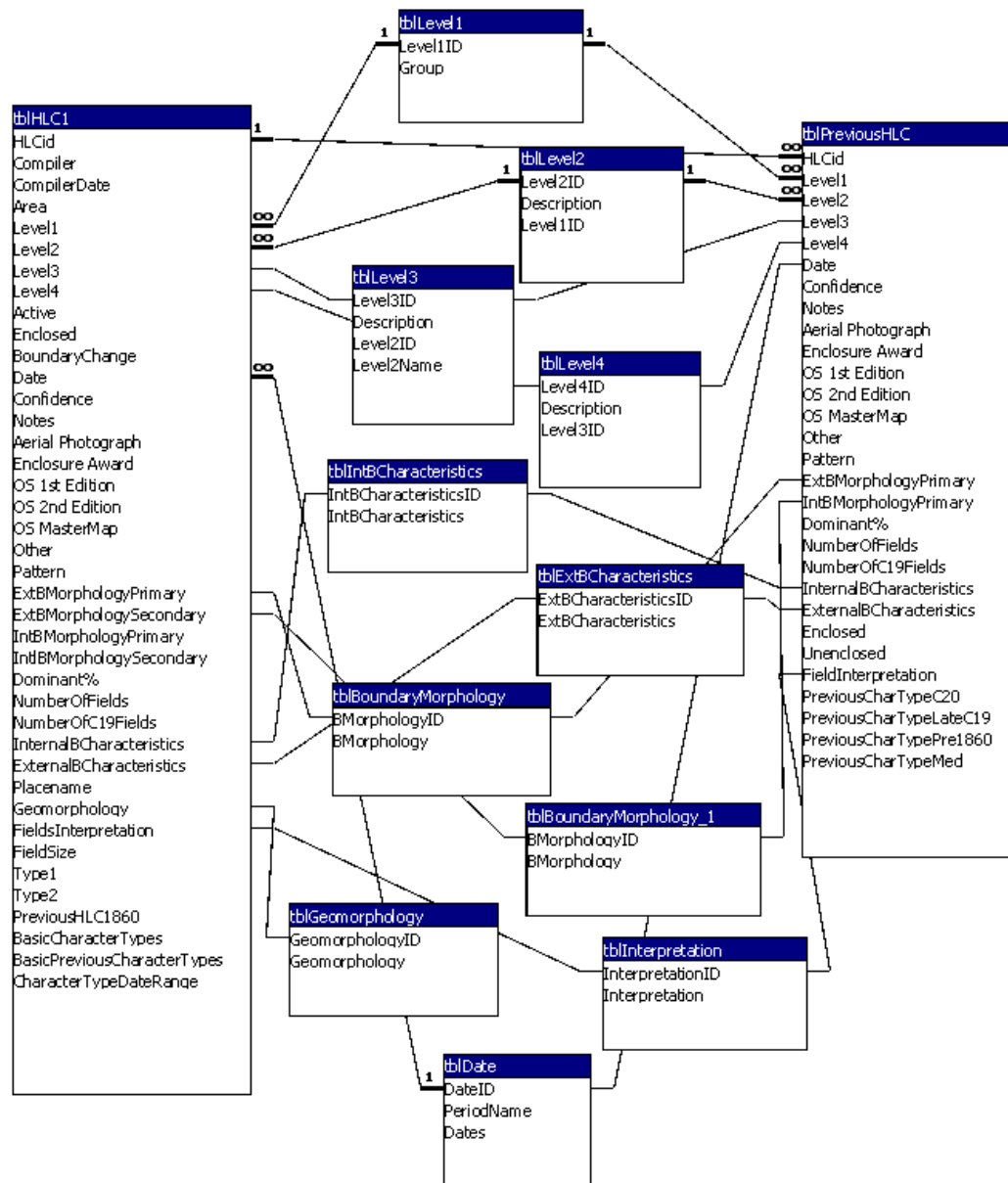
Relationships in HLC database
