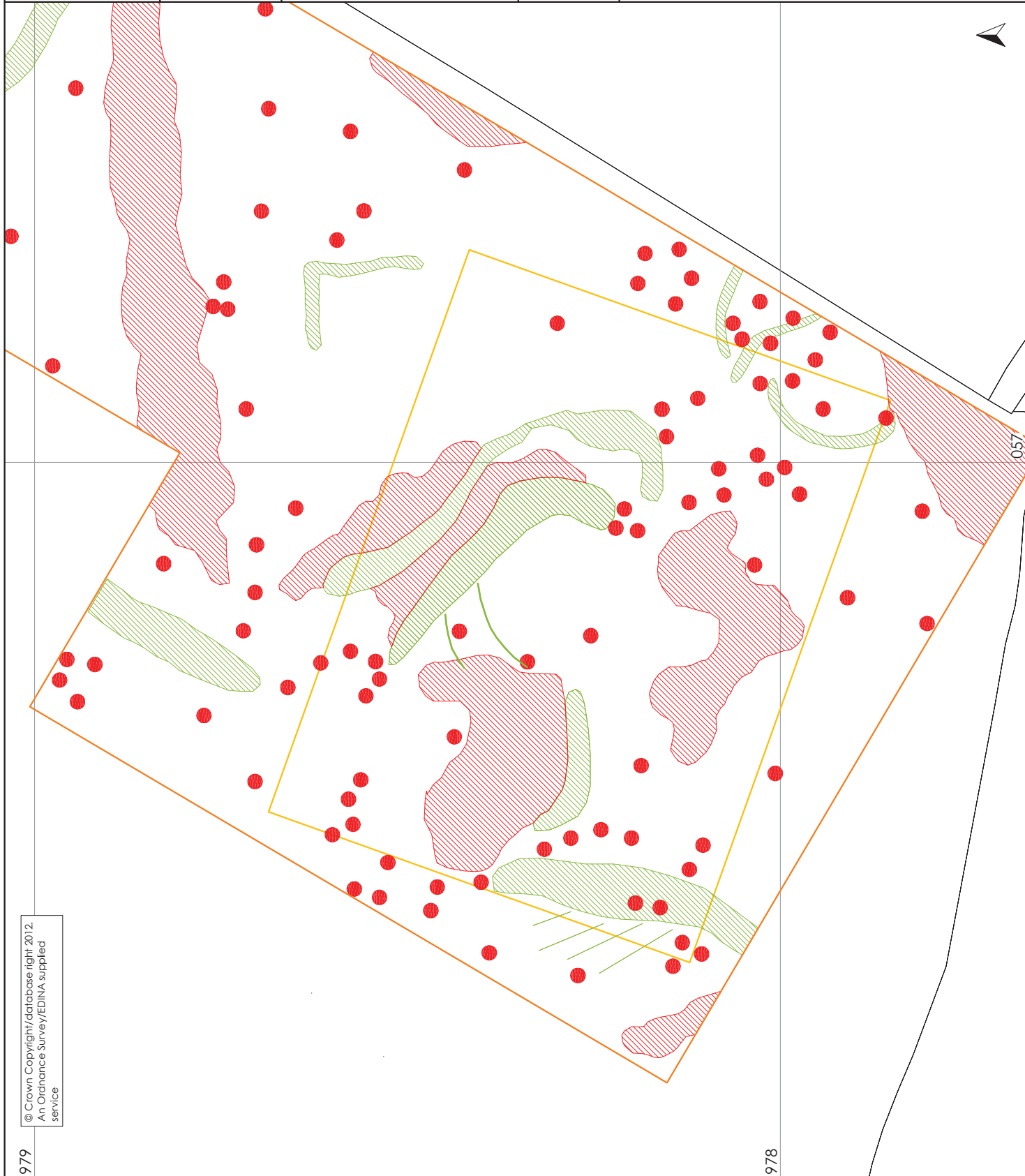
Figure 15: Cogden Hall extract from geomagnetic survey interpretation
