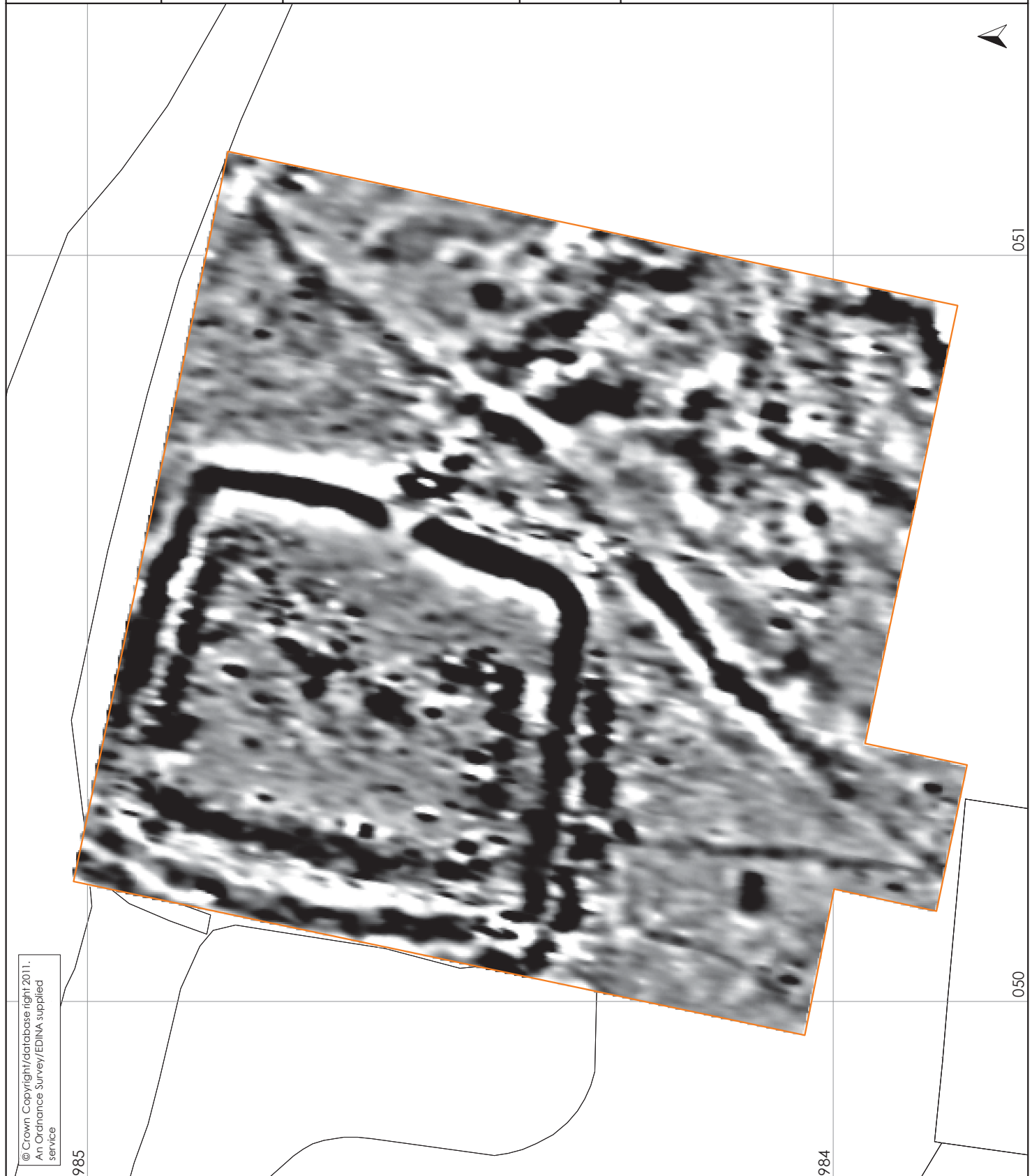
Figure 3: Grinton Mound East geomagnetic survey (filtered data)
