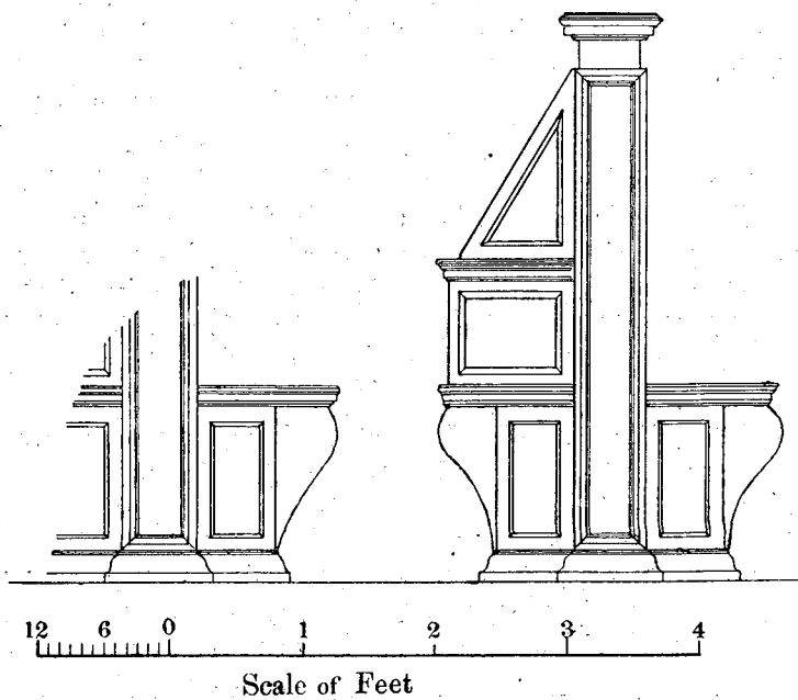
FIG. 7. Elevation of book-desks and reader's seats, Biblioteca Laurentiana, Florence.
