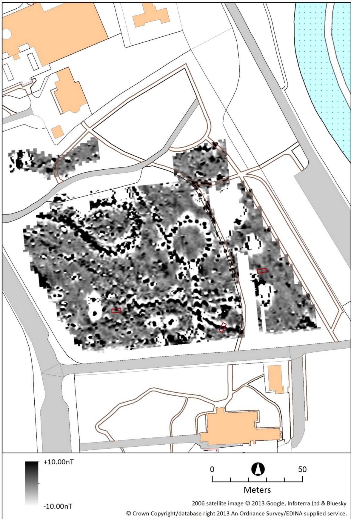
Figure 27: Results of the 2007 gradiometer survey Drewett's Park, Jarrow. (Courtesy of Archaeological Services, Durham University)
