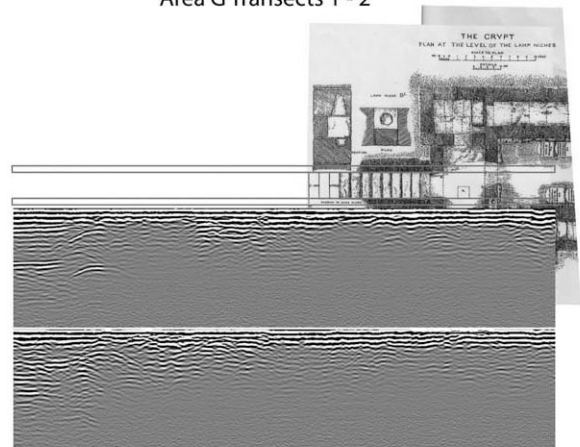
Hexham Abbey GPR Area G Transects 1 - 2
