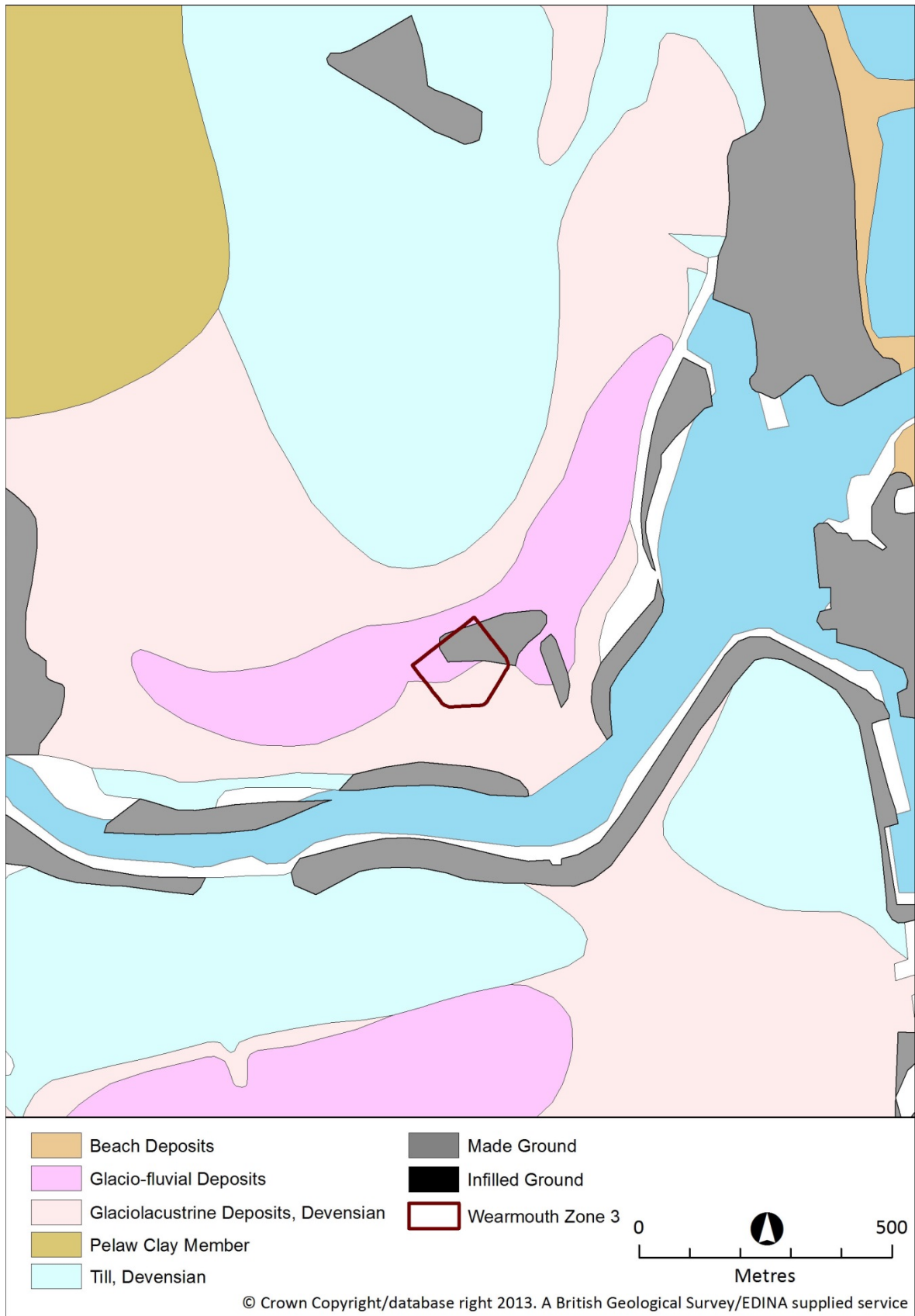
Figure 7: Geology of Wearmouth
