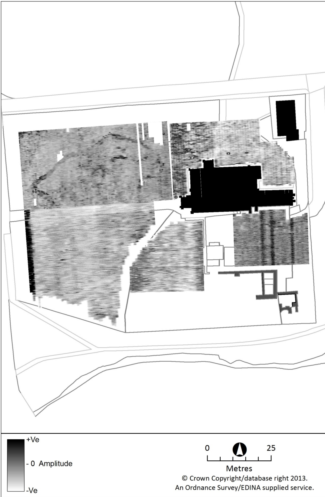
Figure 72: GPR survey results, St Paul's Church, Jarrow, 2009 – depth c.250cm
