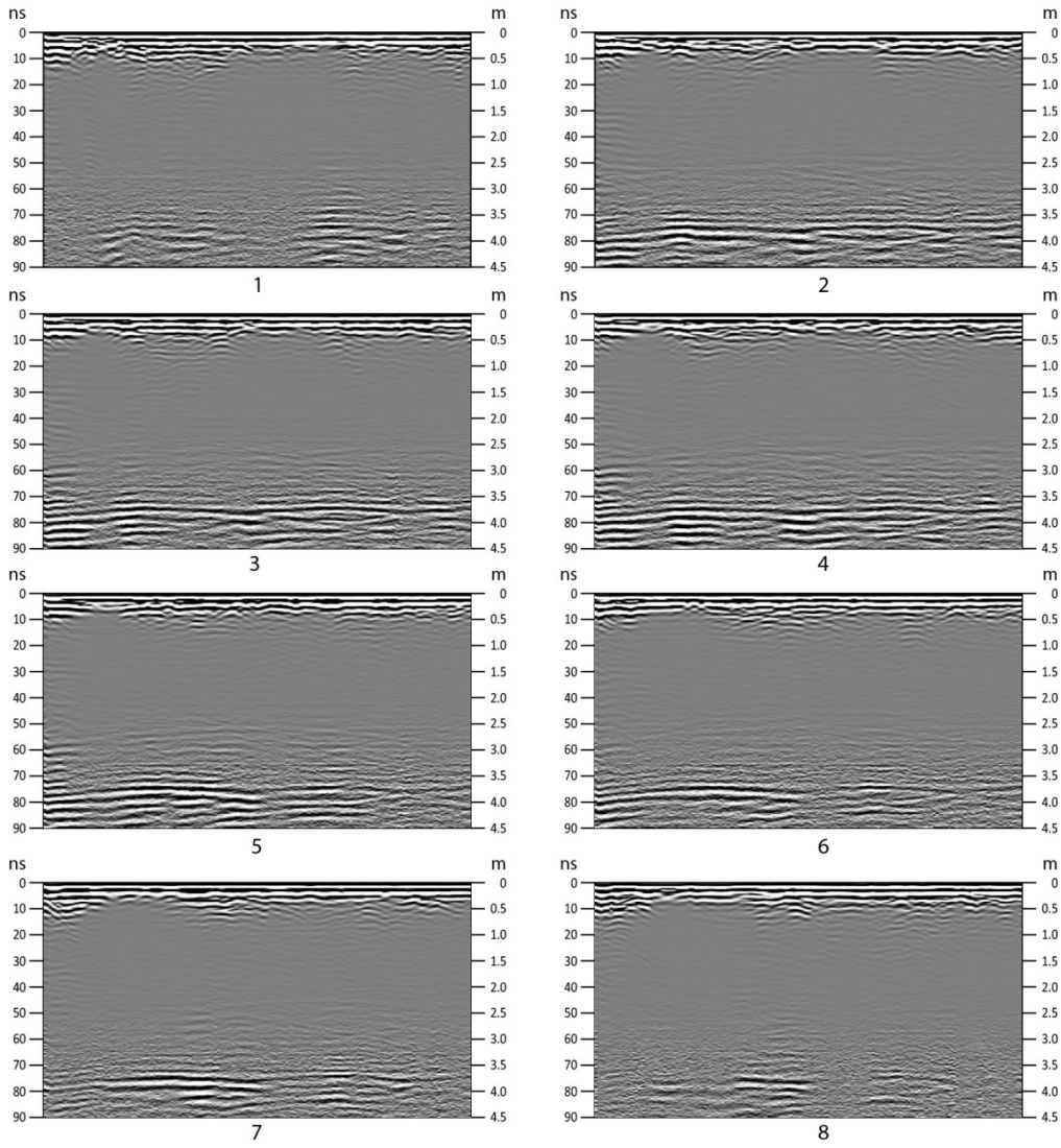
Figure 76: Internal GPR survey St Paul's Church, Jarrow, 2010. Profiles for Area A
