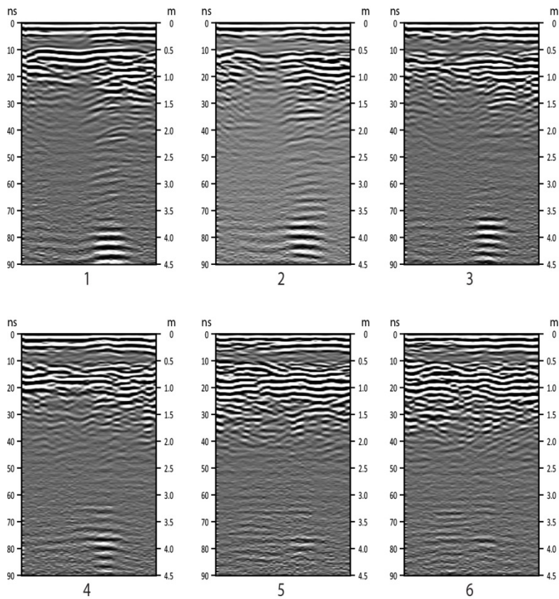
Figure 82: Internal GPR survey St Paul's Church, Jarrow, 2010. Profiles for Area H.
