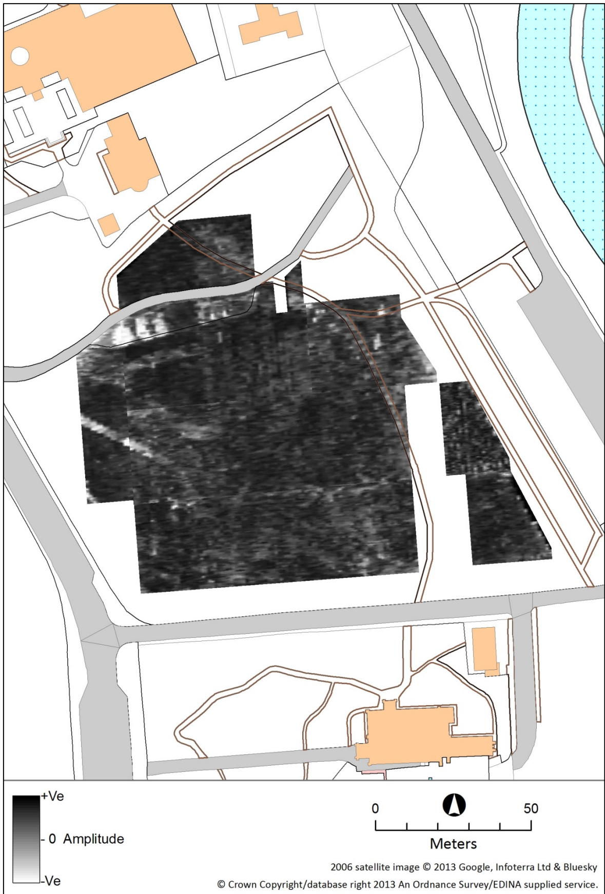
Figure 45: GPR results Drewett's Park, 2008 – depth c. 2.0 metres
