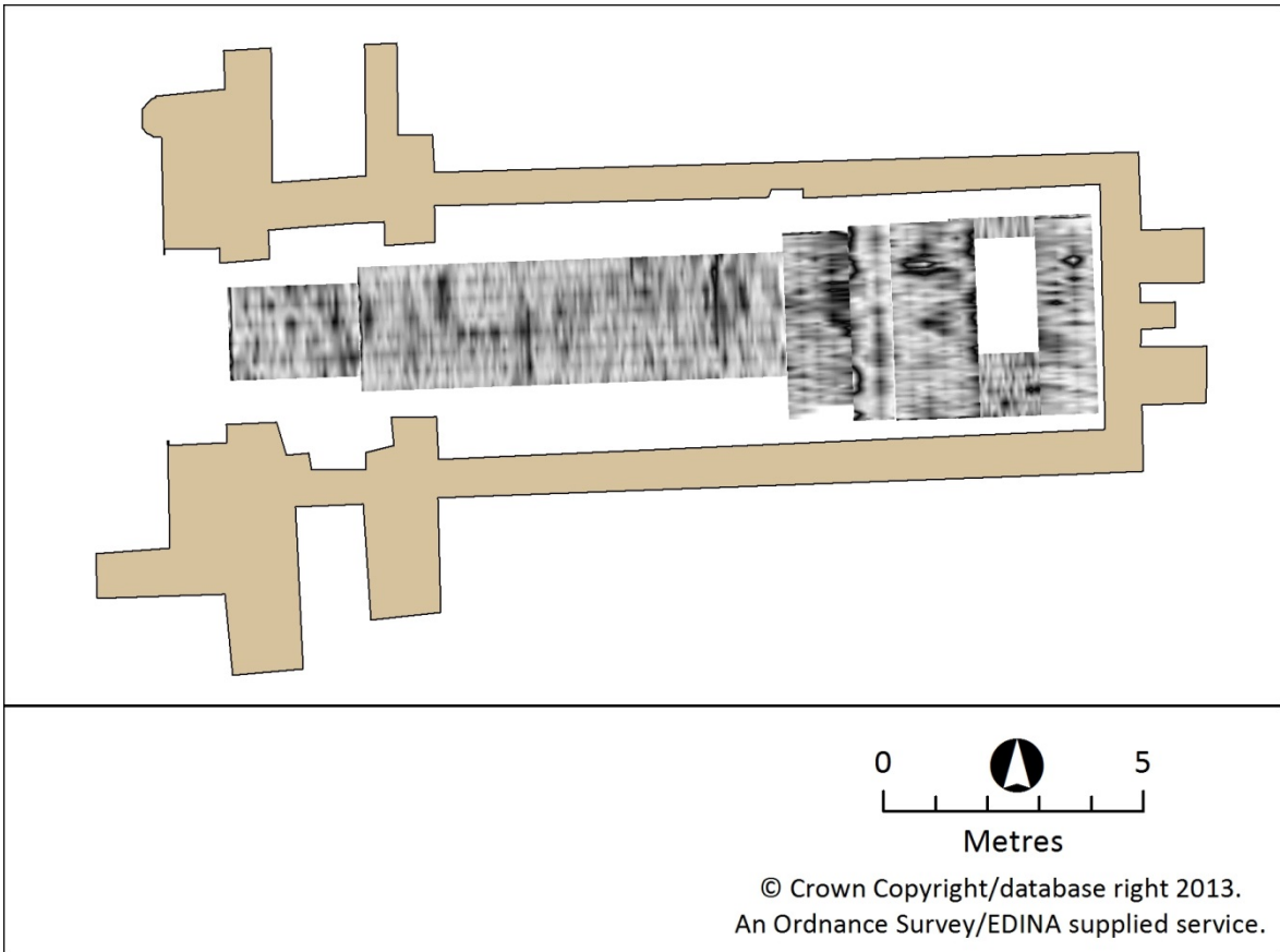
Figure 95: Internal GPR survey St Paul's Church, Jarrow, 2010. Plot at c.325cm
