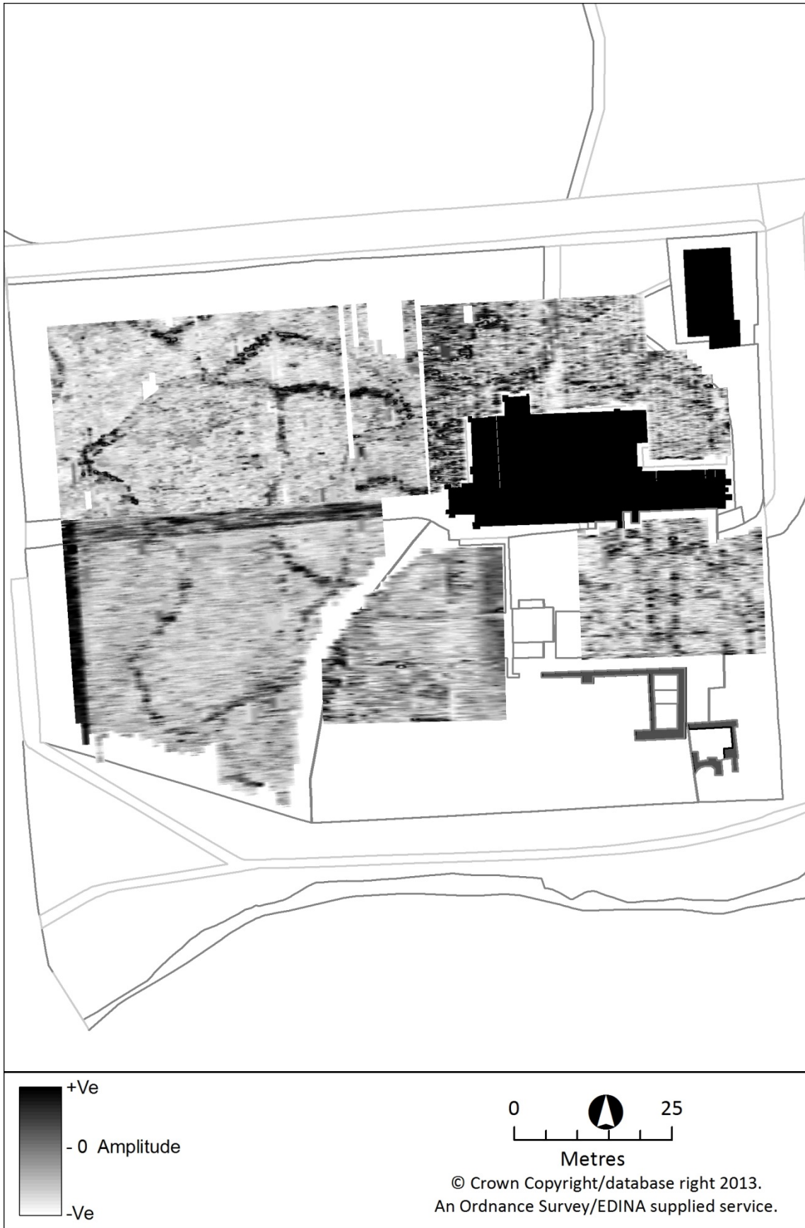
Figure 65: GPR survey results, St Paul's Church, Jarrow, 2009 – depth c.50cm
