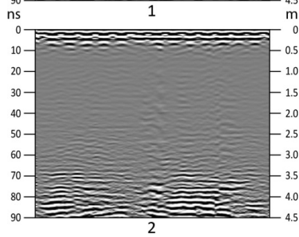
Figure 77: Internal GPR survey St Paul's Church, Jarrow, 2010. Profiles for Areas B and C.
