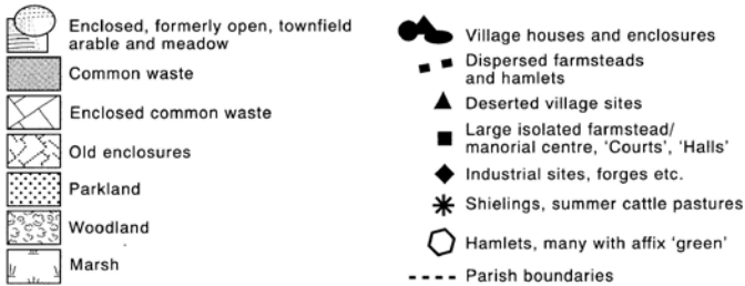
Figure 14: Diagrammatic model of the West Wessex Sub-province
