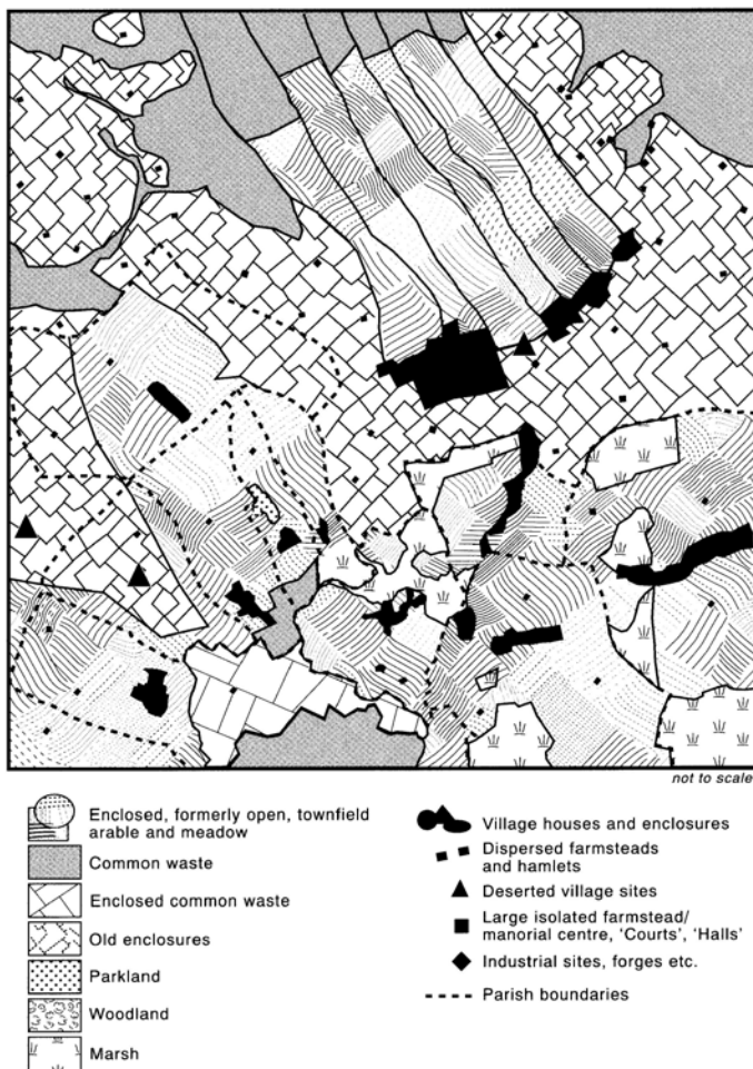
Figure 8: Diagrammatic model of the East Yorkshire Sub-province
