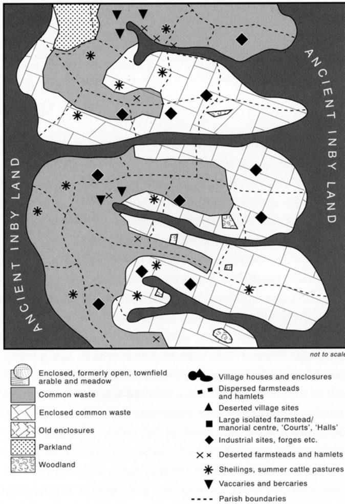
Figure 15: Diagrammatic model of the Cheviots and Northern and Southern Pennines Sub-provinces
