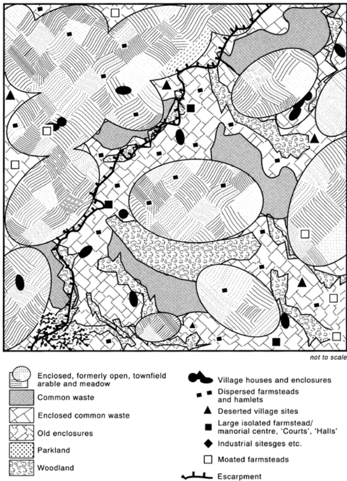
Figure 13: Diagrammatic model of the Cotswold Scarp and Vale Sub-province
