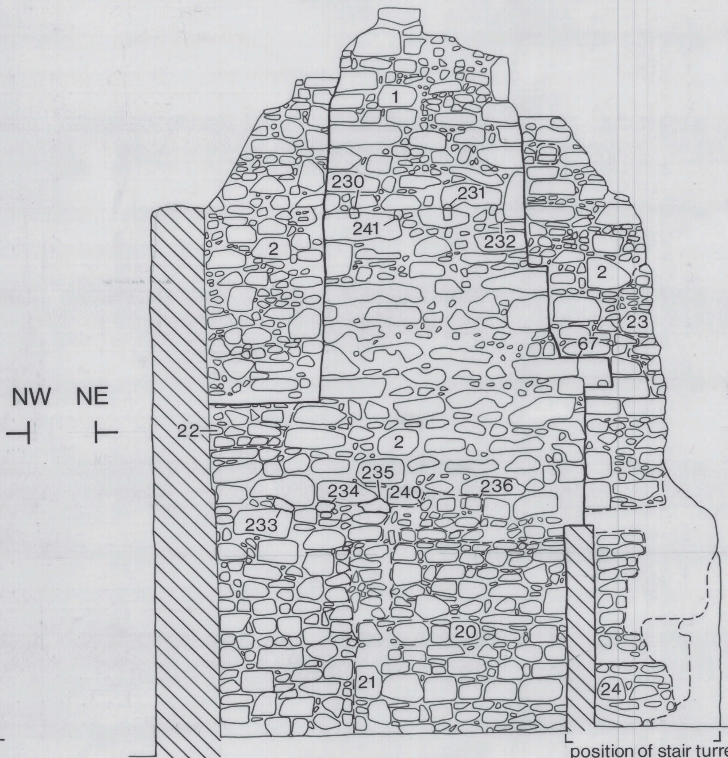
NW Elevation
