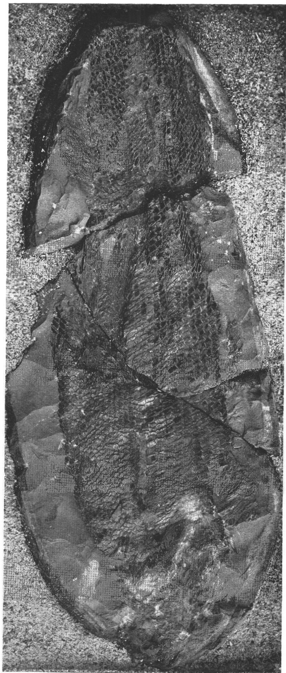
Fossil Fish.
