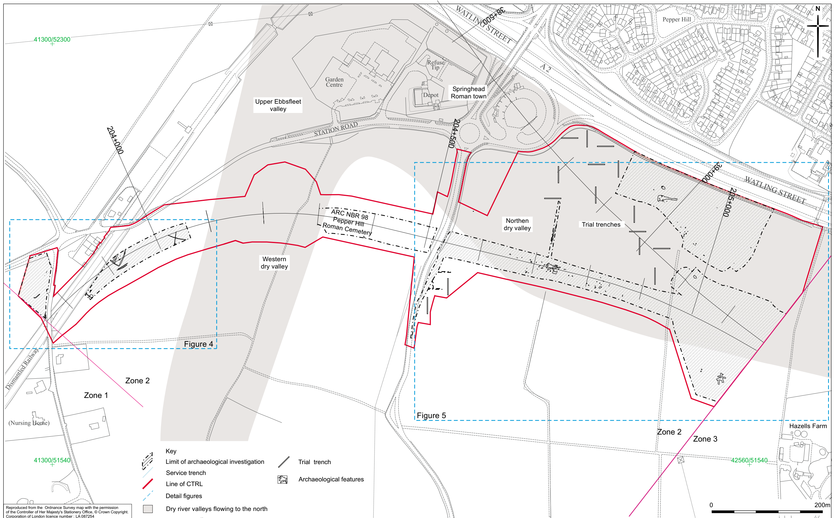
Figure 3. Areas of investigation and dry valleys
