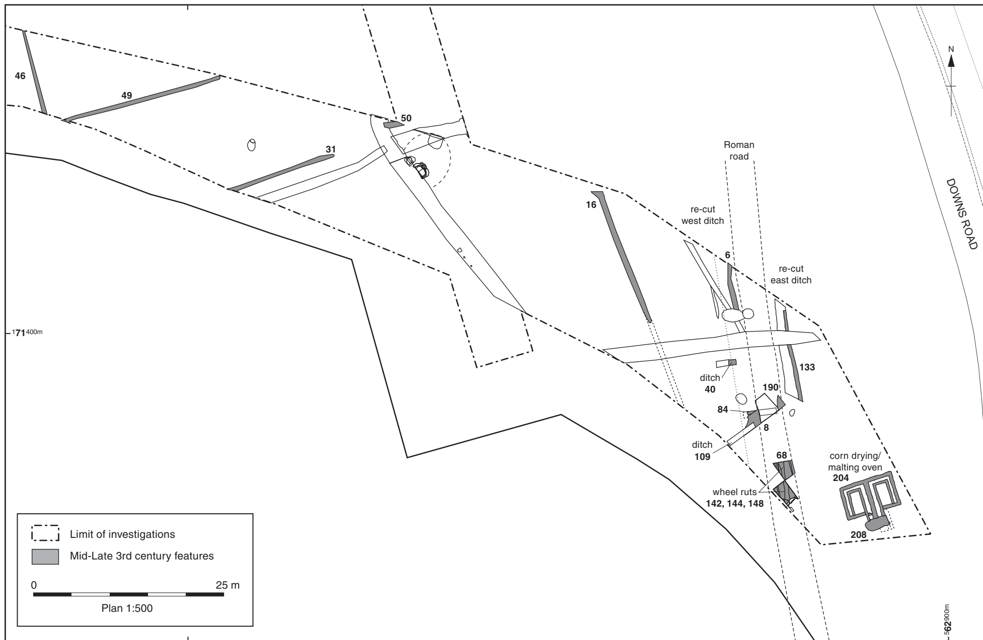
Figure 21: Phase I plan of the Roman road and associated features in the mid-late 3rd century AD
