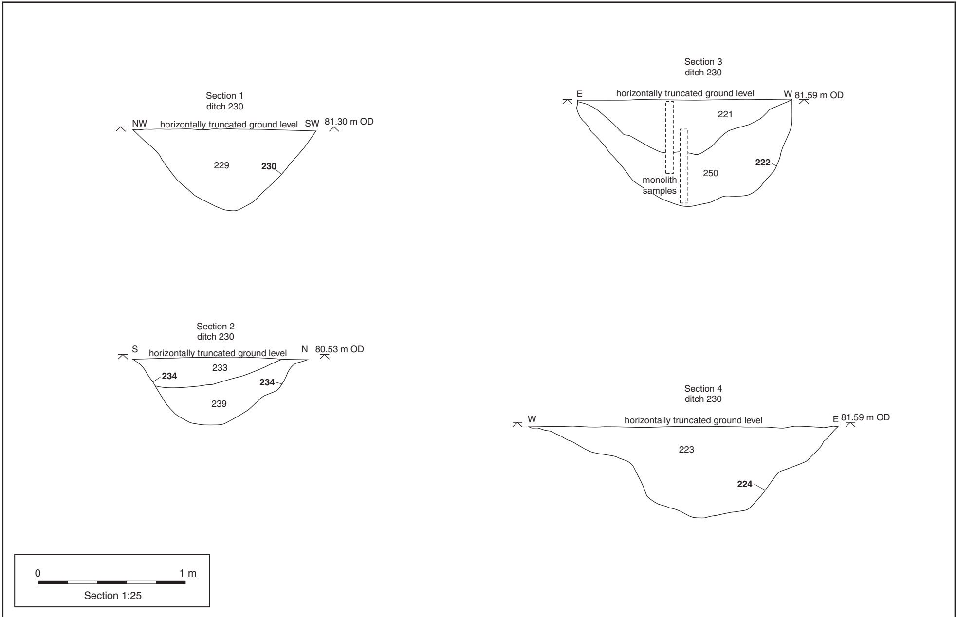
Figure 4: Profiles of the ring ditch; refer to Figure 3 for section locations
