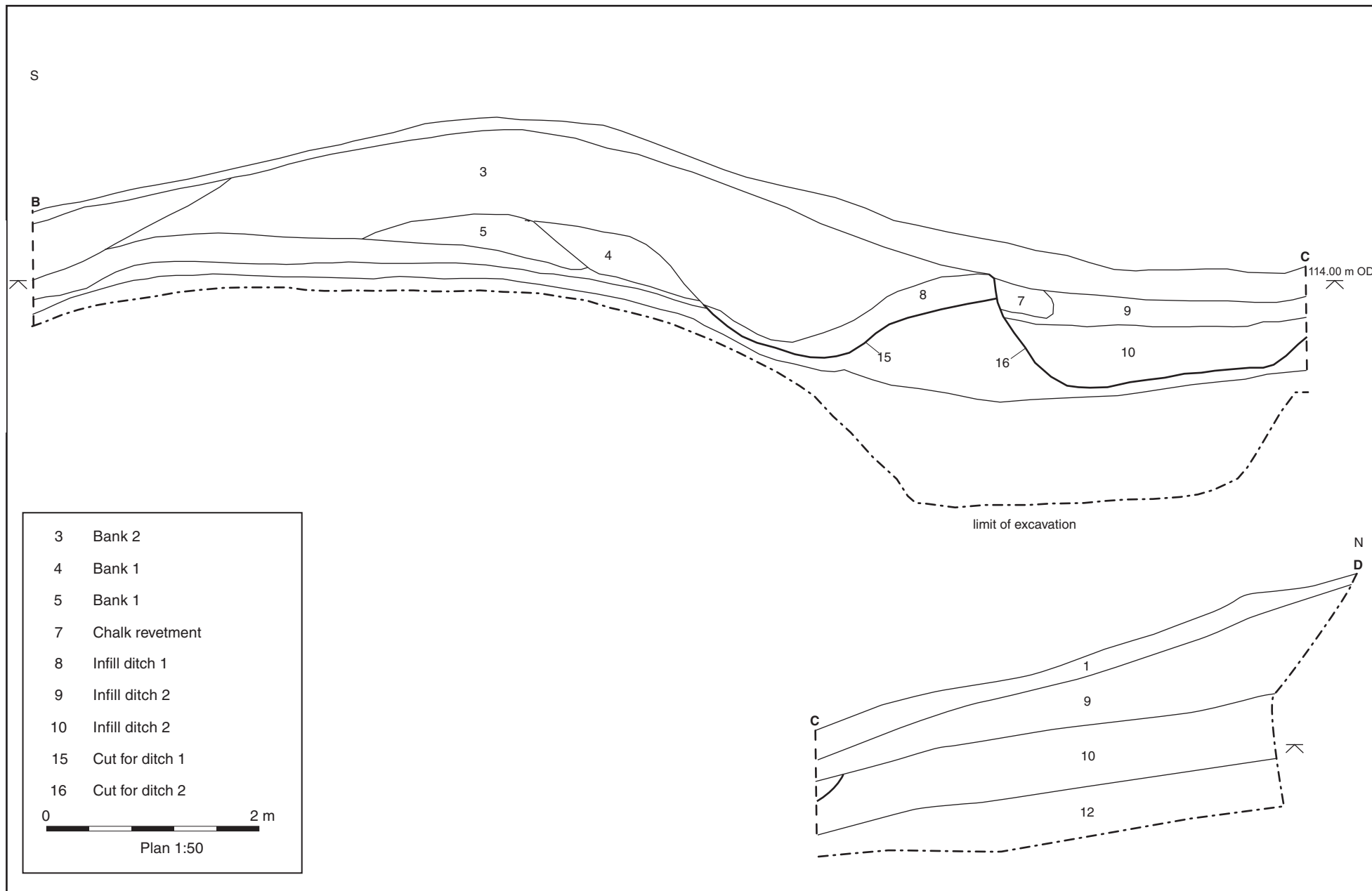
Figure 9: Section 1 through the 18th century park pale or ha-ha
