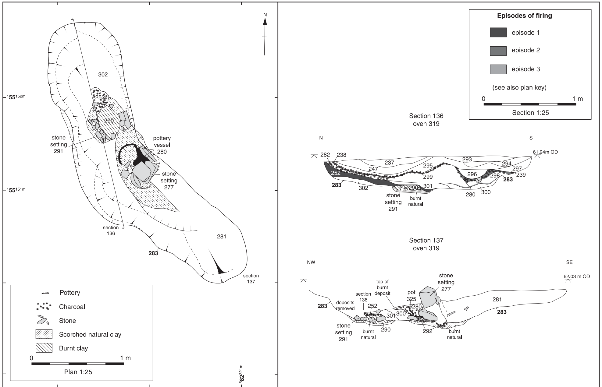
Figure 6: Snarkhurst Wood, oven 319 plan and selected sections
