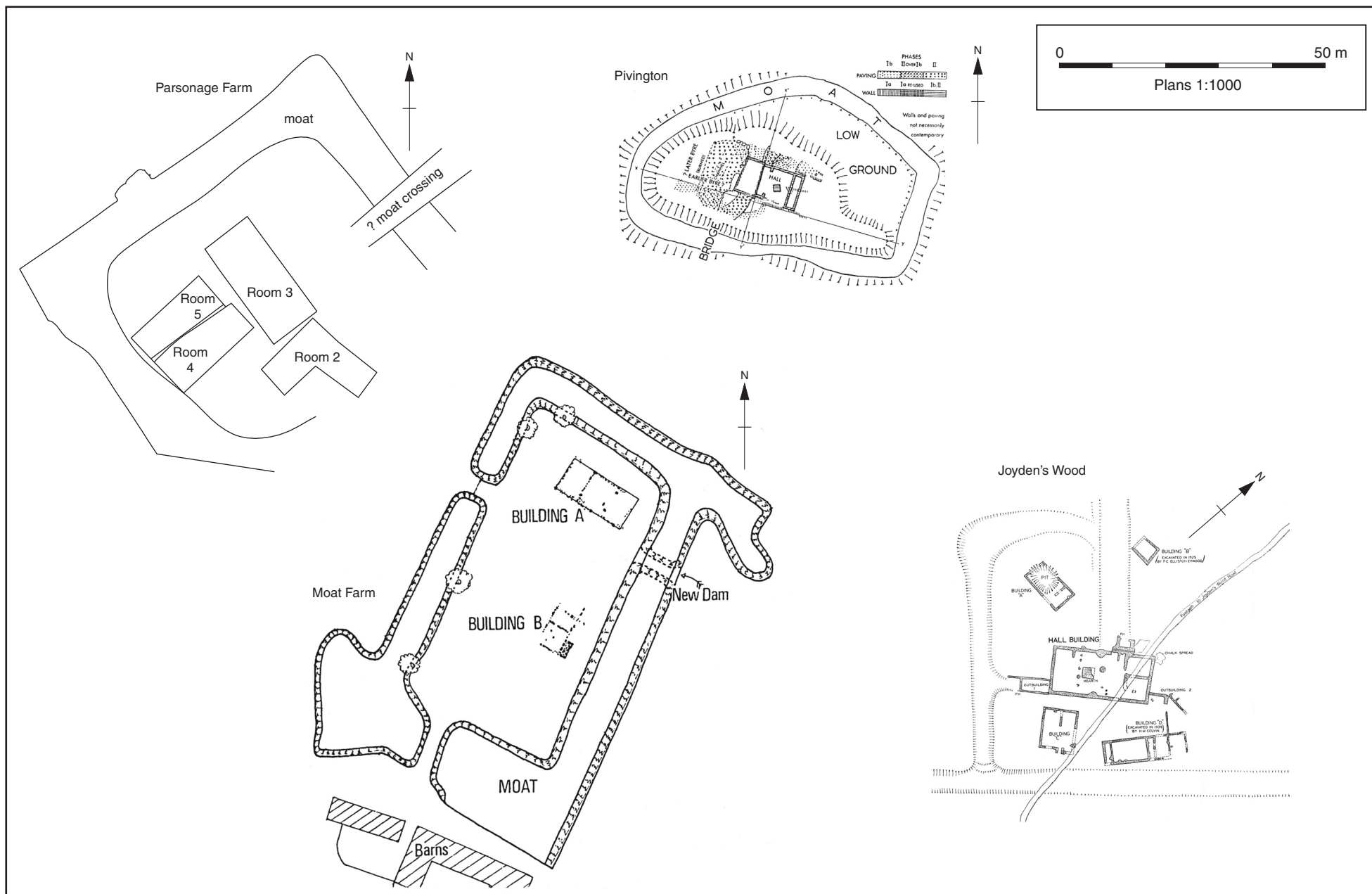
Figure 12: Comparative plans of Parsonage Farm, Pivington, Moat Farm and Joyden's wood, Bexley
