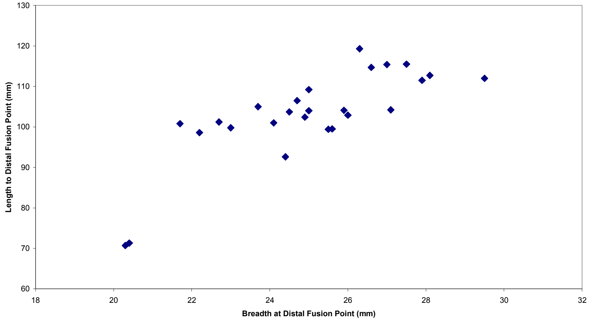
Figure 2: G73 Sheep Metacarpal Shaft Length and Breadth at Distal Fusion Point Measurements
