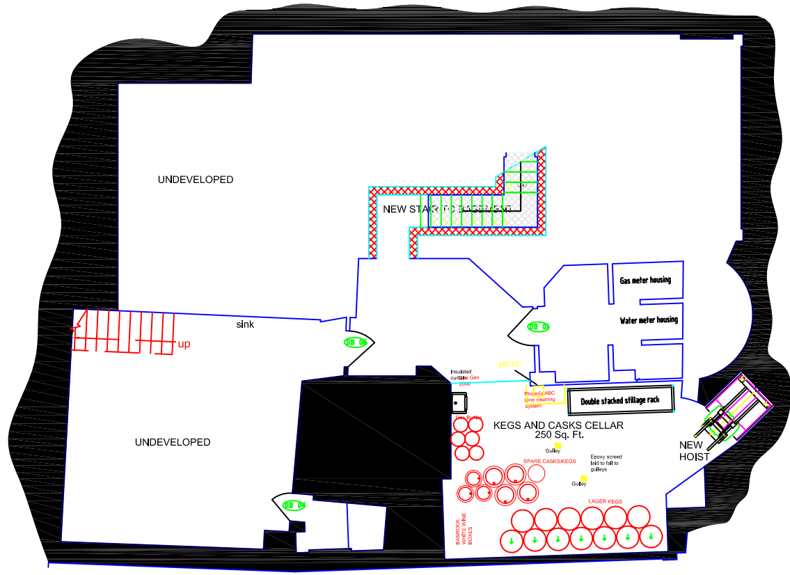
BASEMENT PLAN
