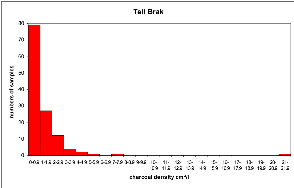
Figure 5 Tell Brak: Frequency histogram showing charcoal densities
