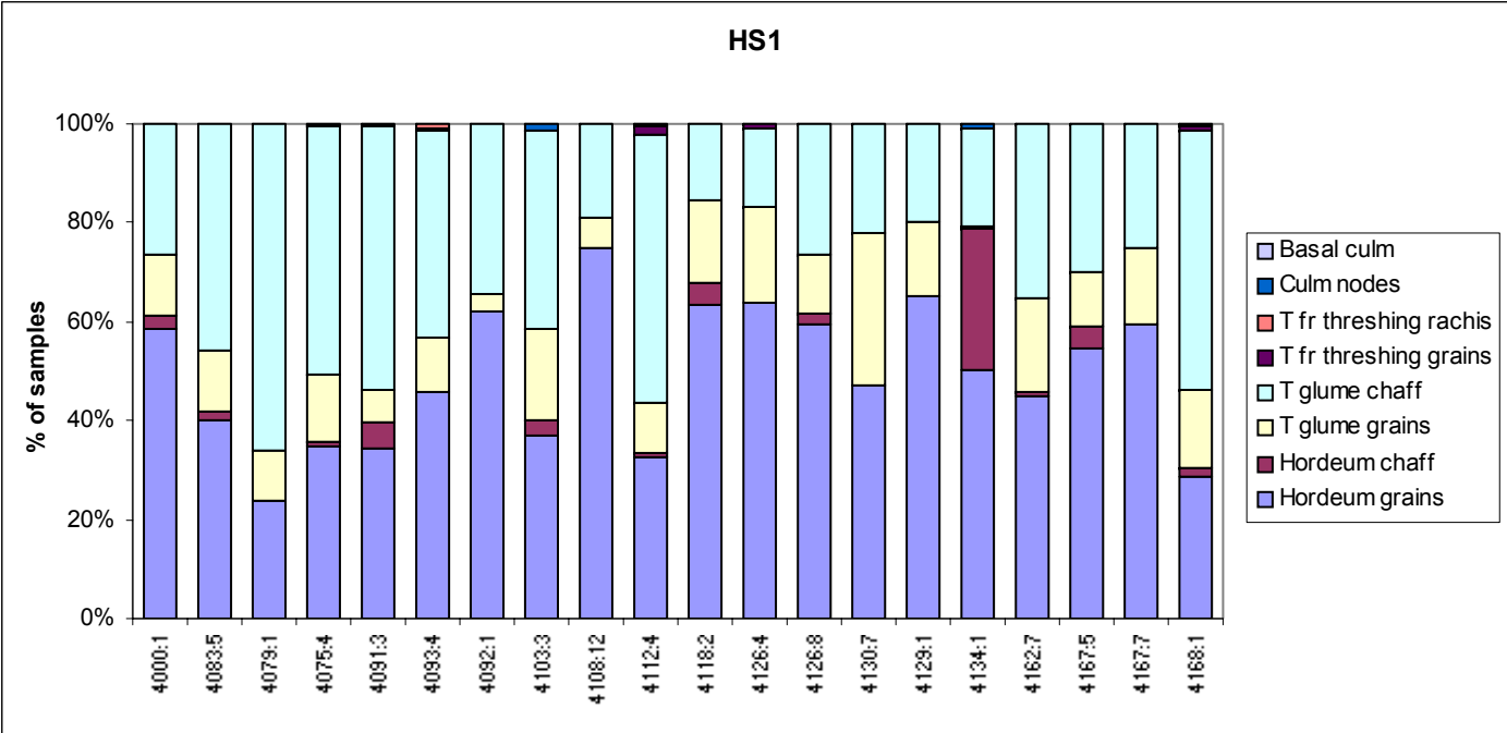
Figure 23 Tell Brak: Cereal proportions by trench – HS1, HS3
