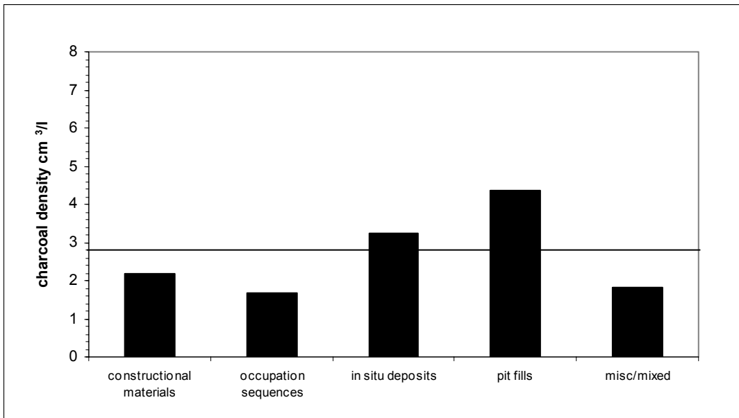
Figures 56-59 Kilise Tepe: Mean charcoal densities by context class
