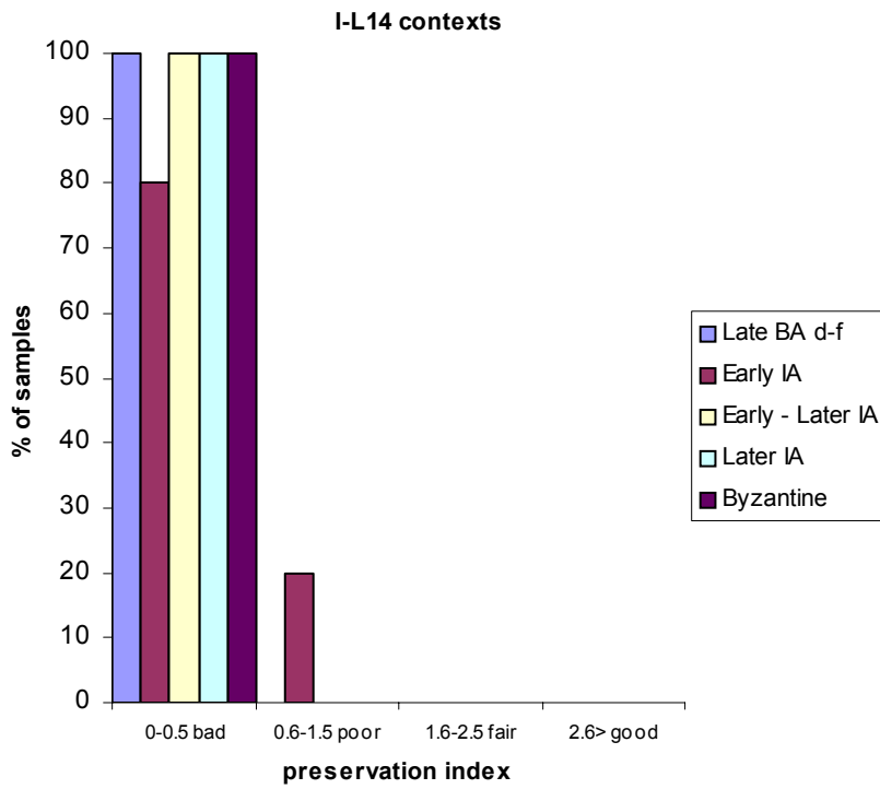
Figure 63 Kilise Tepe: Preservation indices by vertical context – I-L14 samples
