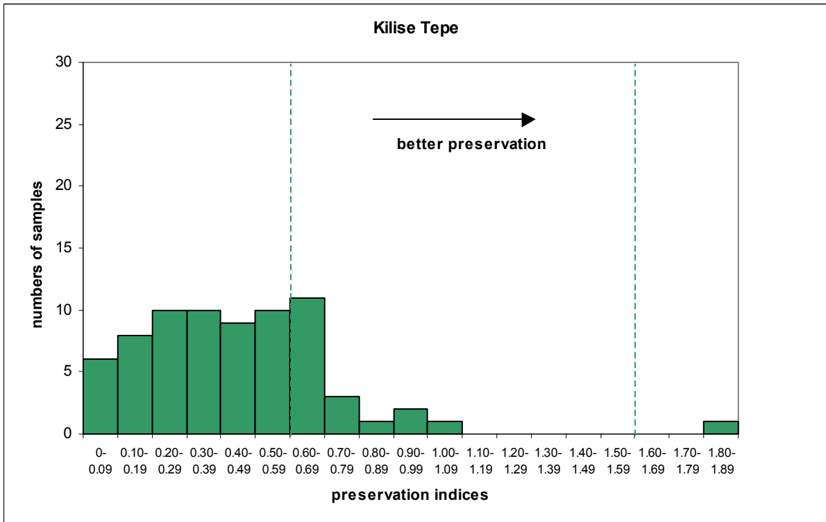
Figure 69 Kilise Tepe: Frequency histogram showing preservation indices
