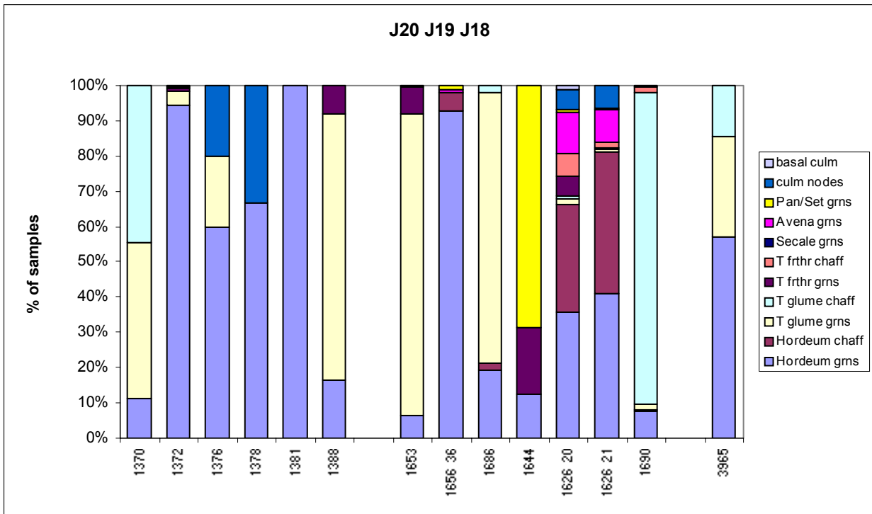
Figure 76 Kilise Tepe: Cereal proportions by trench – J, K
