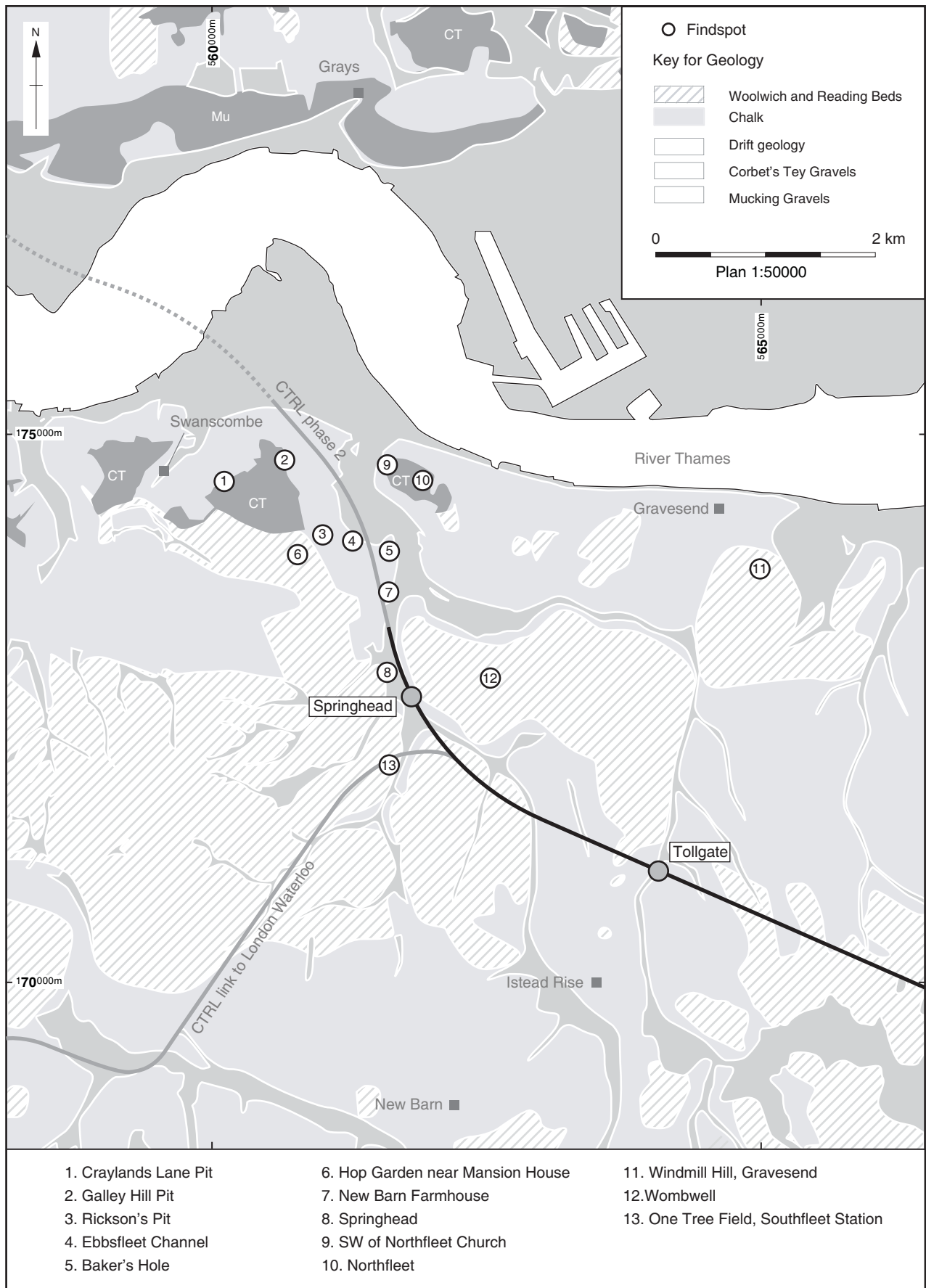
Figure 5: Scheme wide flint report, Palaeolithic finds from the Ebbsfleet area (after Southern Rivers Palaeolithic Project, Wessex Archaeology) shown against a background of simplified geology
