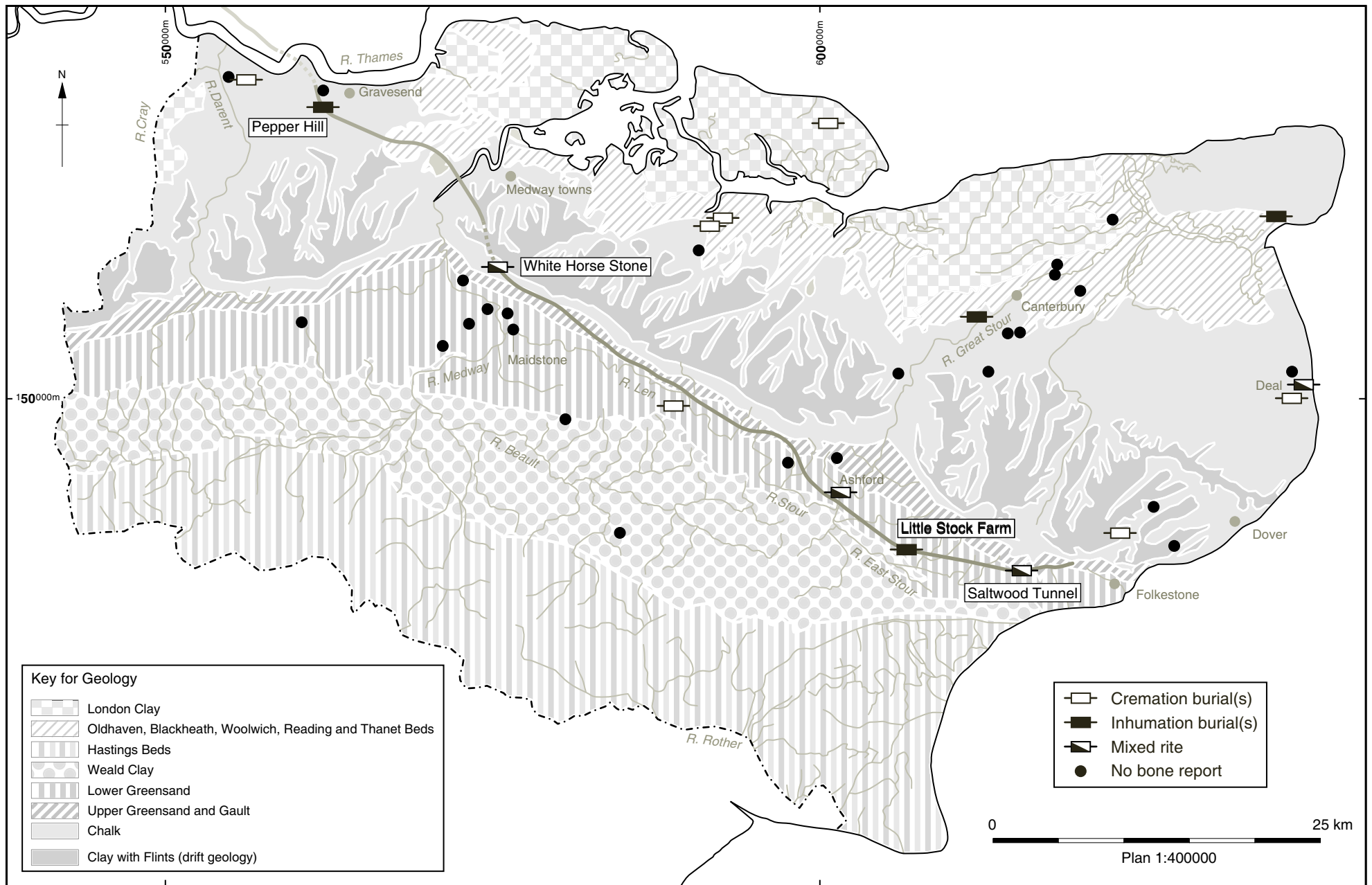
Figure 4: Scheme wide human remains report. Distribution of sites from which Iron Age burials have been recorded against a background of drainage patterns and simplified geology (based on Mays and Anderson 1995, and Lawson and Killingray (eds) 2003)
