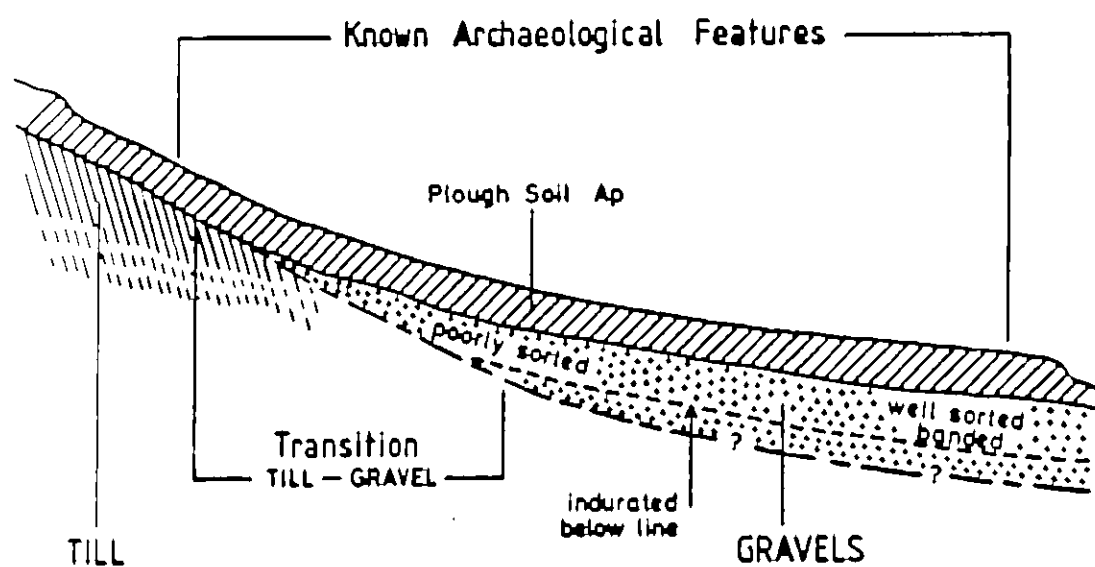
ILL 115 : Excavation site. Schematic section of underlying soils
