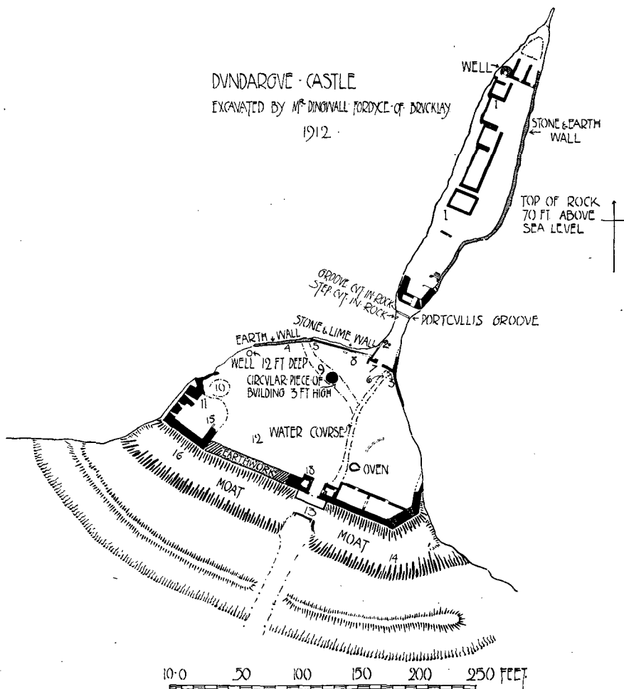
Fig. 1. Plan of Dundargove Castle.
