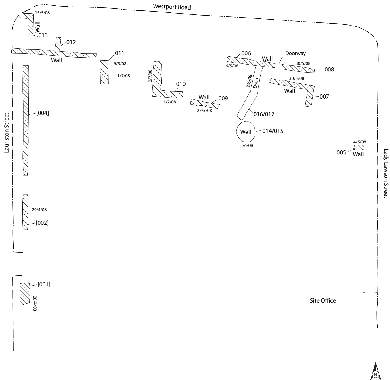
Figure 2: Site Plan
