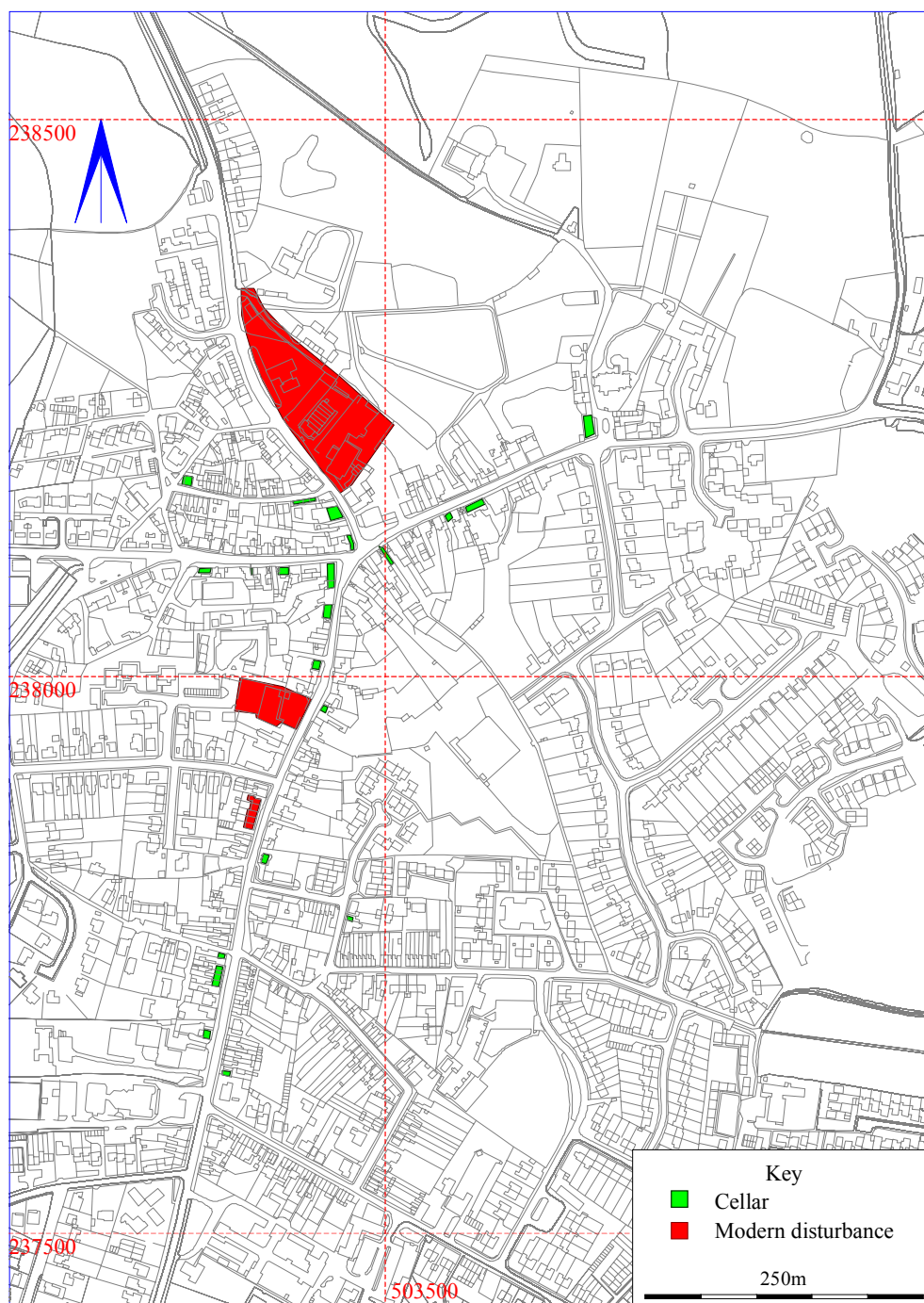
Figure 11: Likely extent of modern disturbance within historical core.
