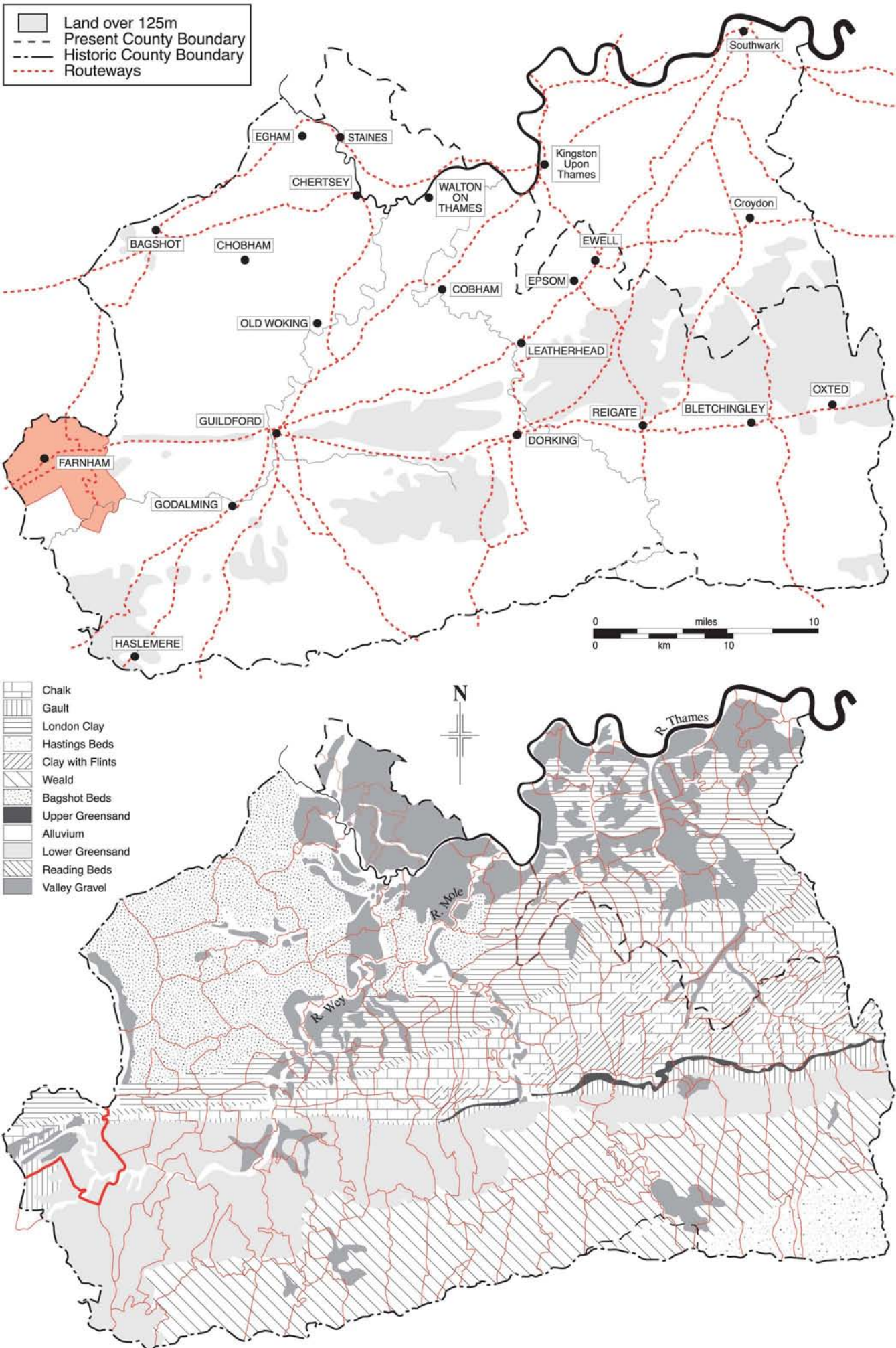
Fig 1 Extensive Urban Survey of Surrey. Top: Farnham, showing the area of the parish and manor. The principal routeways, as shown on 18th century maps, are also shown. Bottom: parishes (about 1823) and drift geology.
