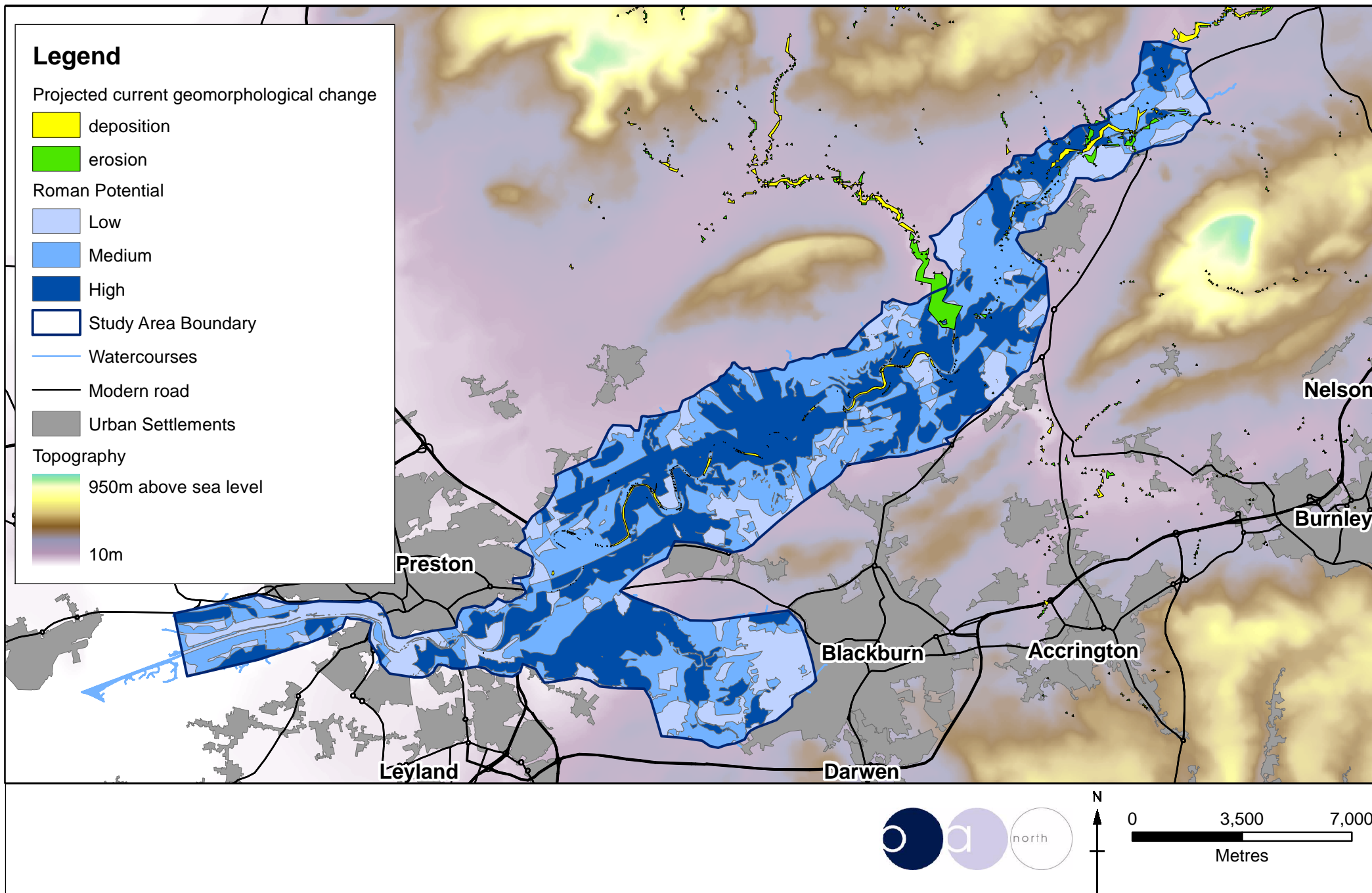
Figure 169: Areas of projected current geomorphological change superimposed on Roman potential
