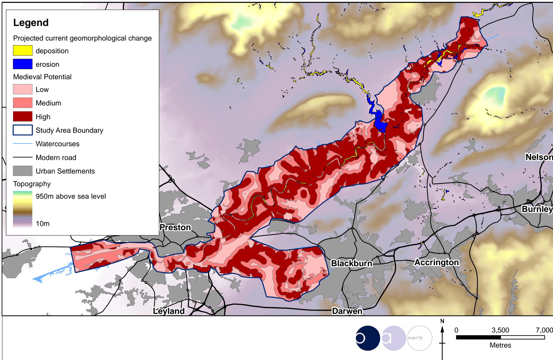
Figure 170: Areas of projected current geomorphological change superimposed on medieval potential
