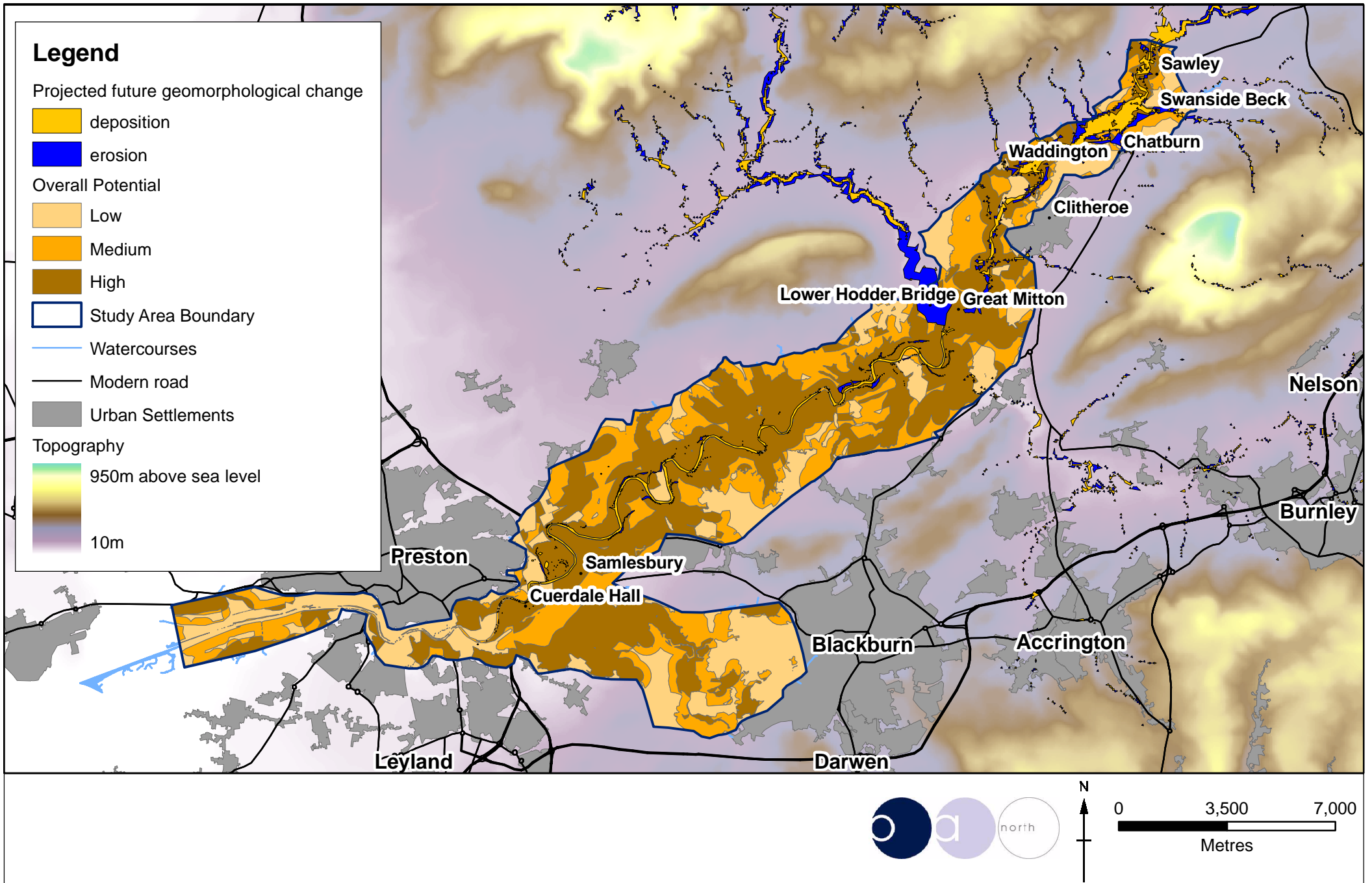
Figure 174: Areas of projected future geomorphological change superimposed on overall archaeological potential
