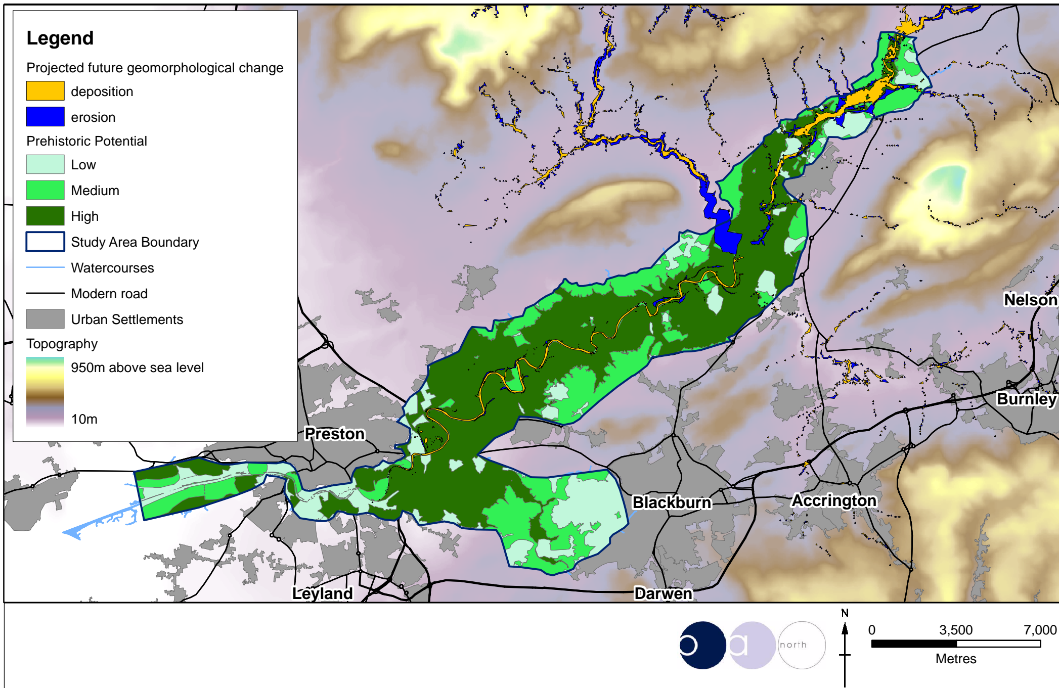
Figure 175: Areas of projected future geomorphological change superimposed on prehistoric potential
