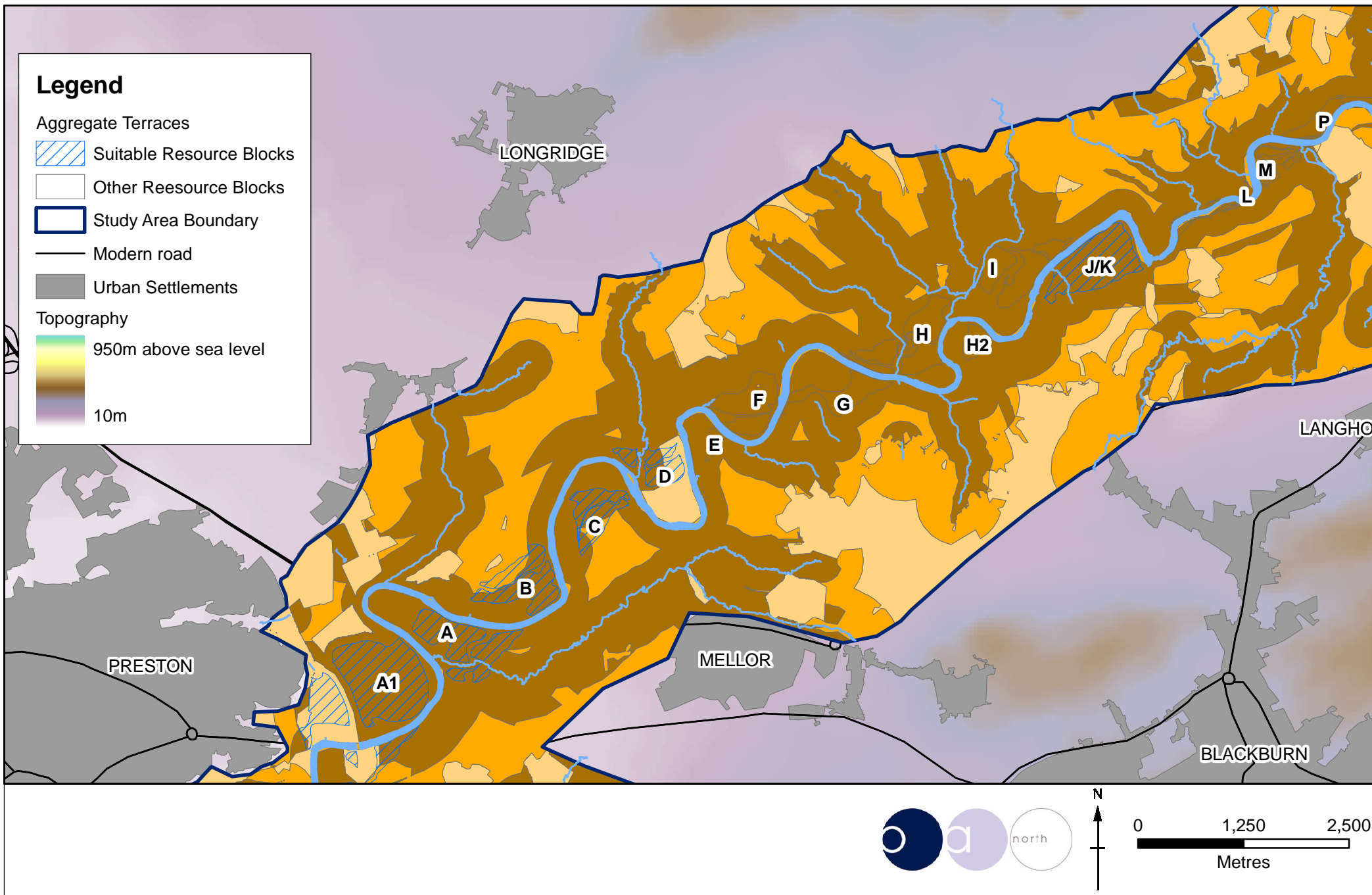
Figure 179: Resource Blocks suitable for aggregate extraction between the M6 and the Calder tributary, superimposed on overall archaeological potential
