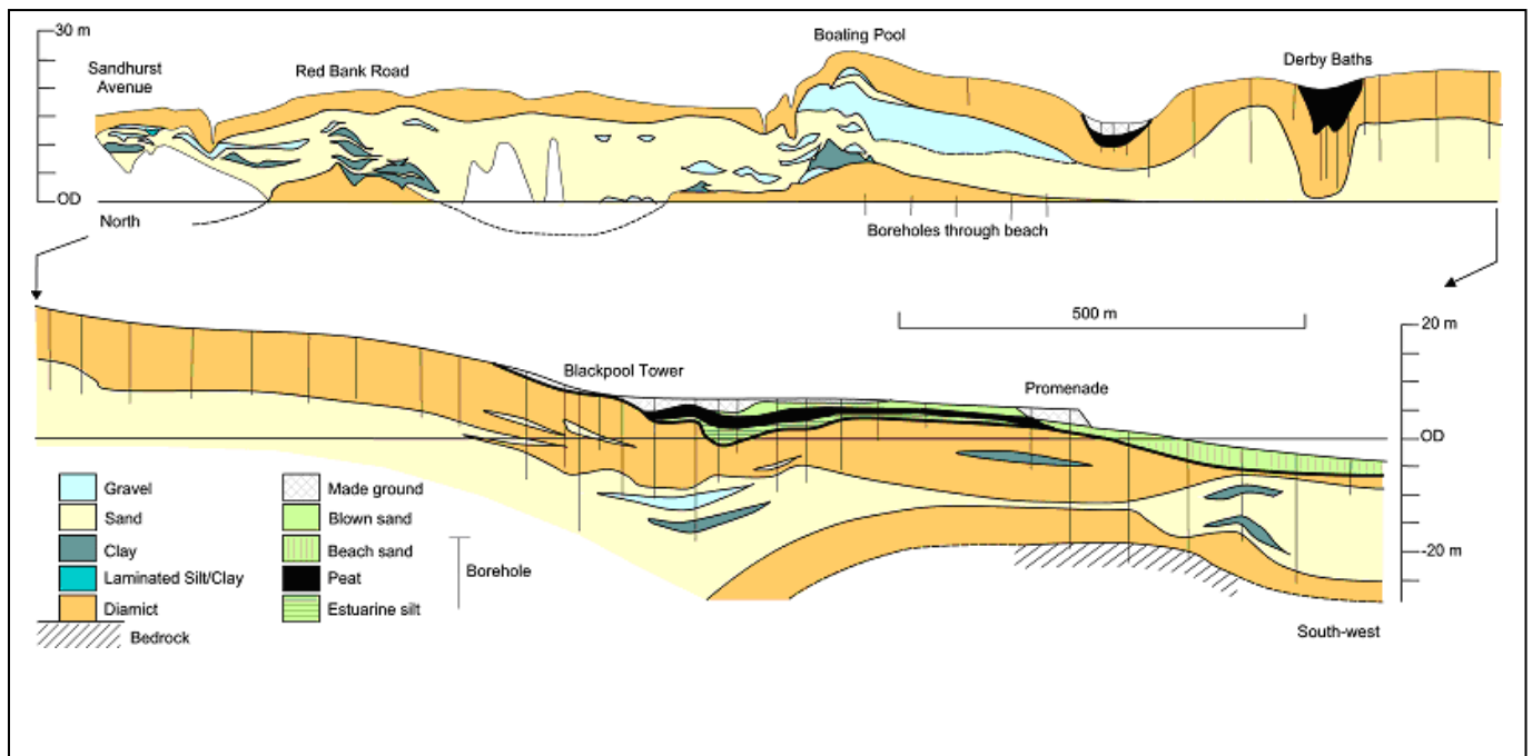
Figure 2: Coastal sections at Blackpool from the researches of Binney (1852) and De Rance (1877a)
